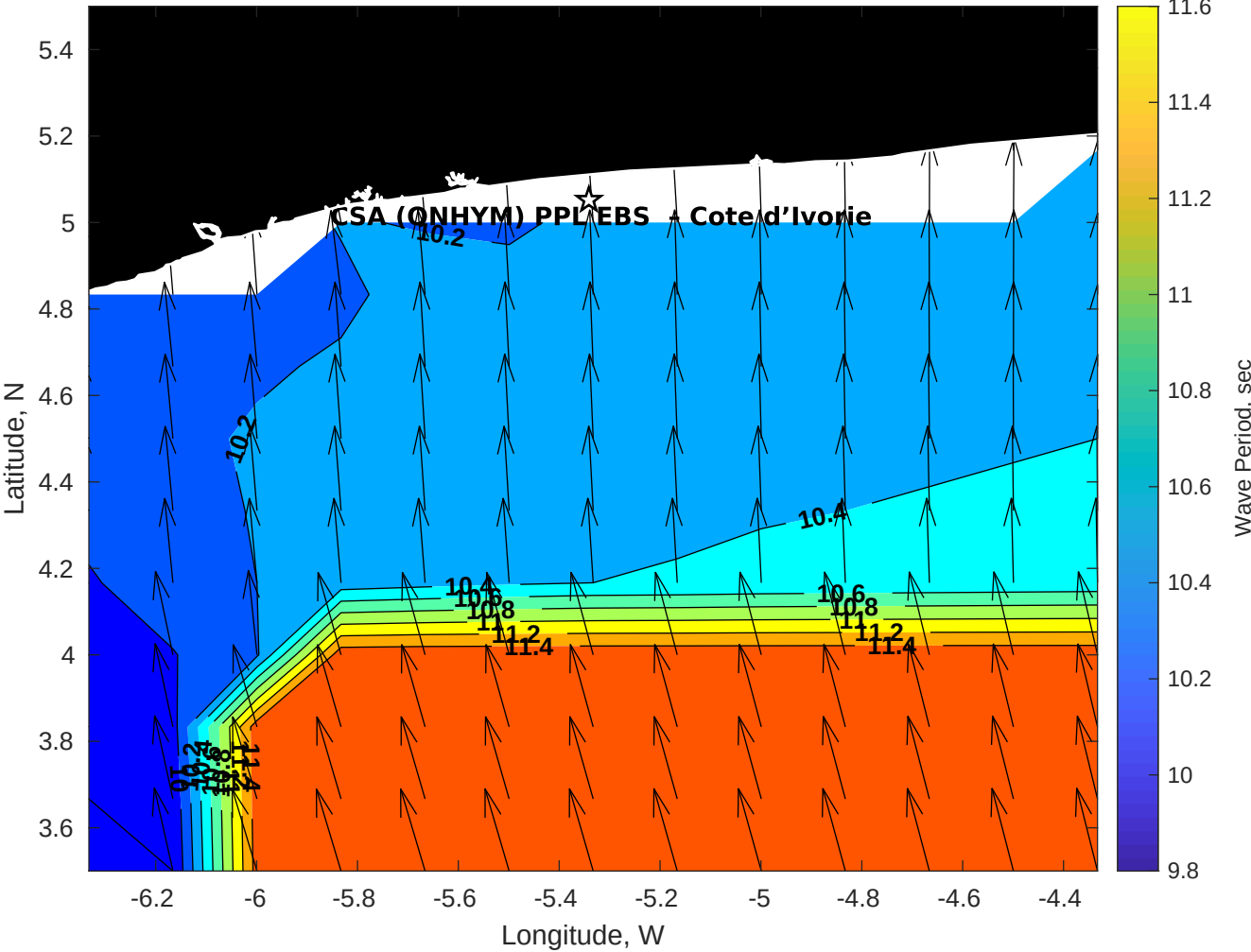
Wave Period (sec) for CSA (ONHYM) PPL EBS - Cote d'Ivoire at 16-May-2025 09:00:00
