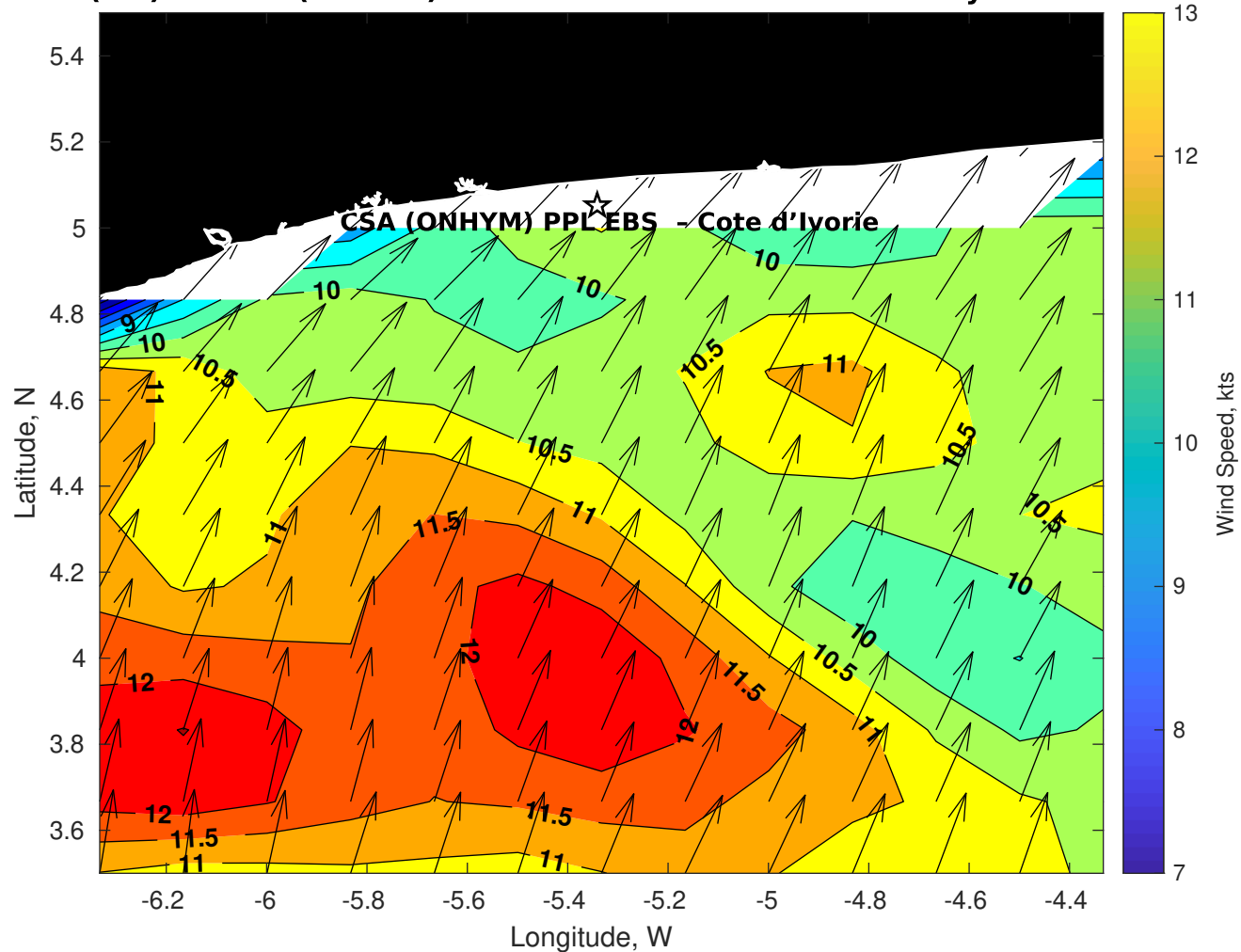
Winds (kts) for CSA (ONHYM) PPL EBS - Cote d'Ivoire at 16-May-2025 09:00:00
