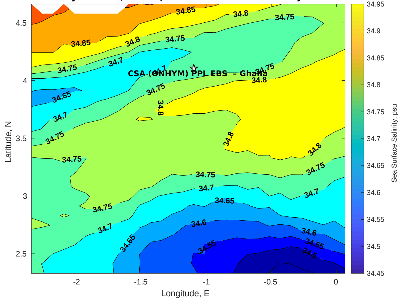
Surface Salinity for CSA (ONHYM) PPL EBS - Ghana at 15-May-2025 00:00:00
