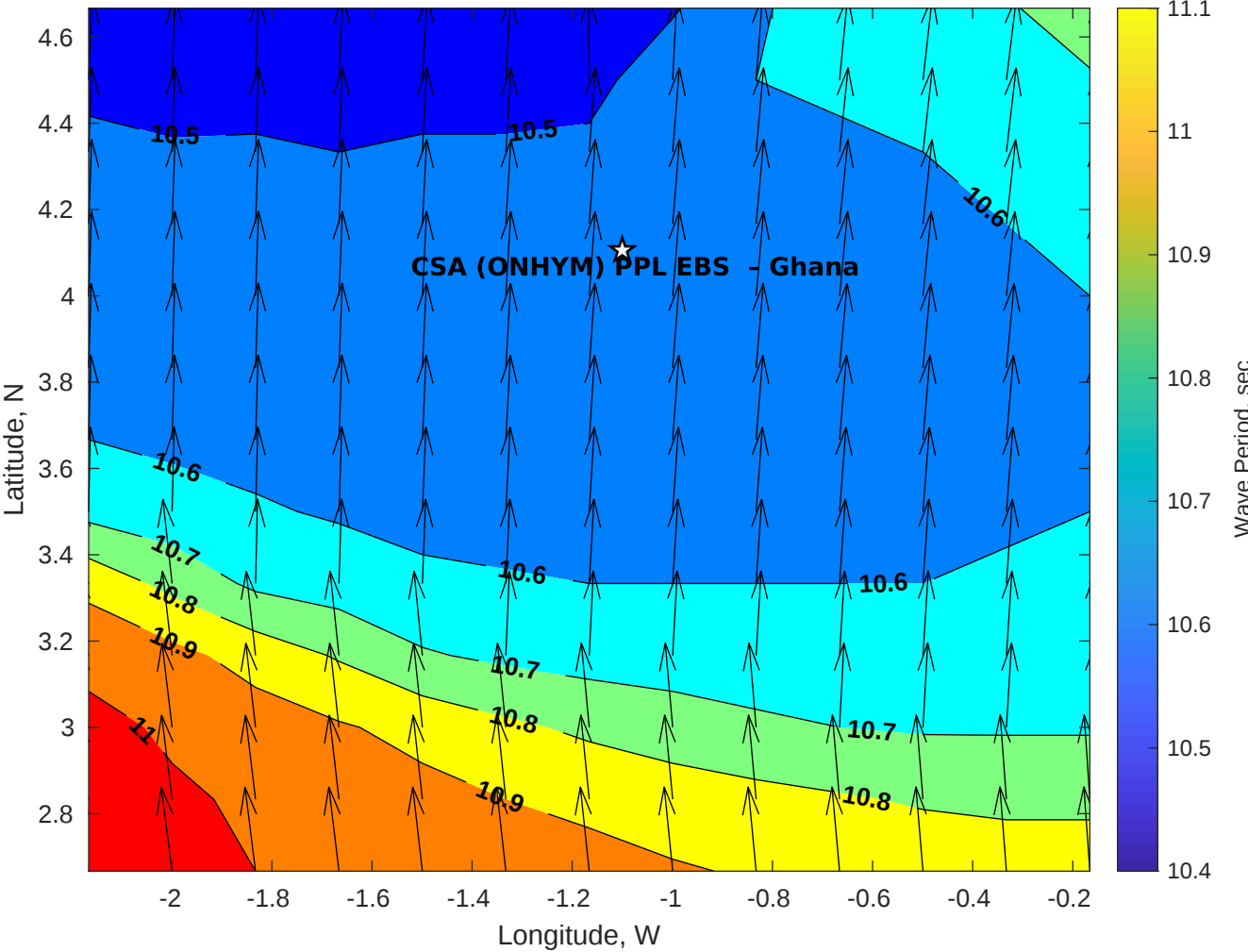
Wave Period (sec) for CSA (ONHYM) PPL EBS - Ghana at 16-May-2025 09:00:00
