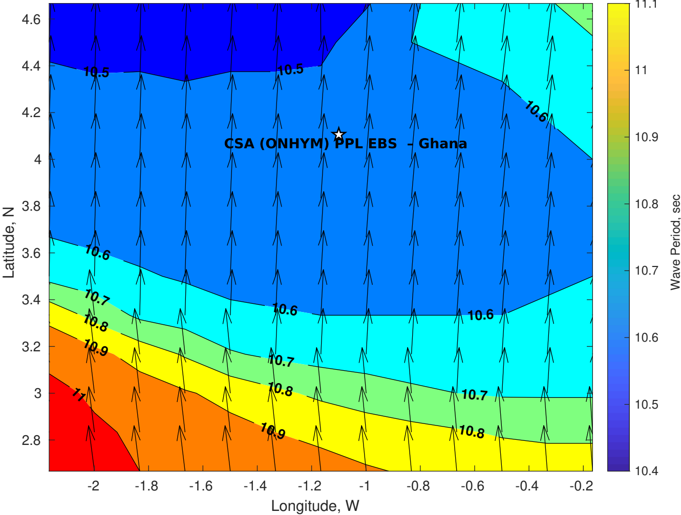
Wave Period (sec) for CSA (ONHYM) PPL EBS - Ghana at 16-May-2025 09:00:00
