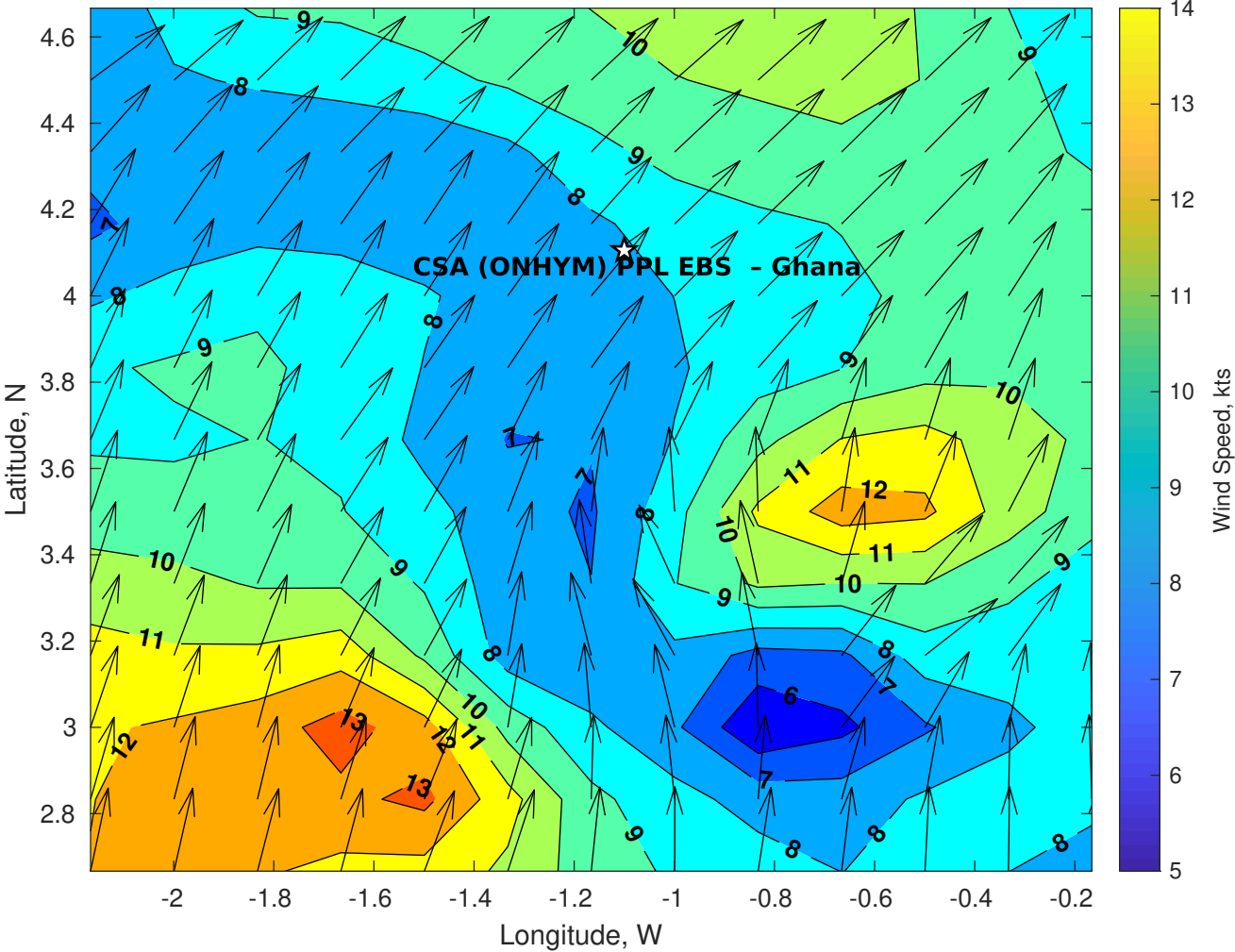
Winds (kts) for CSA (ONHYM) PPL EBS - Ghana at 16-May-2025 09:00:00
