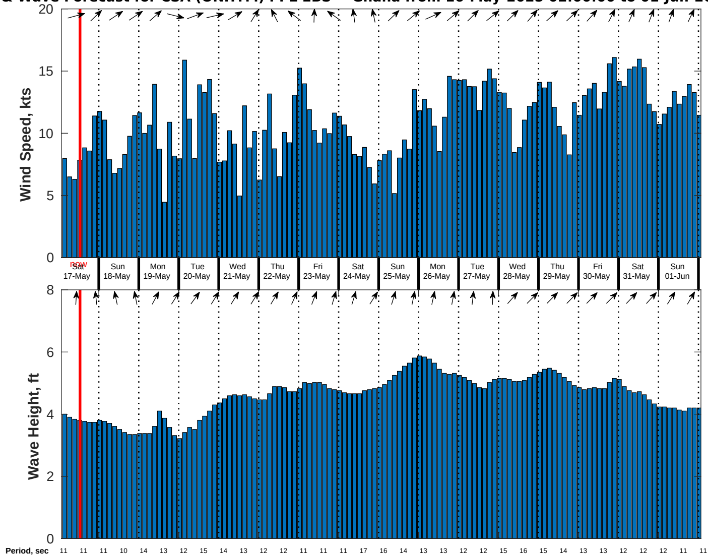
Wind & Wave Forecast for CSA (ONHYM) PPL EBS - Ghana from 16-May-2025 02:00:00 to 01-Jun-2025 02:00:00
