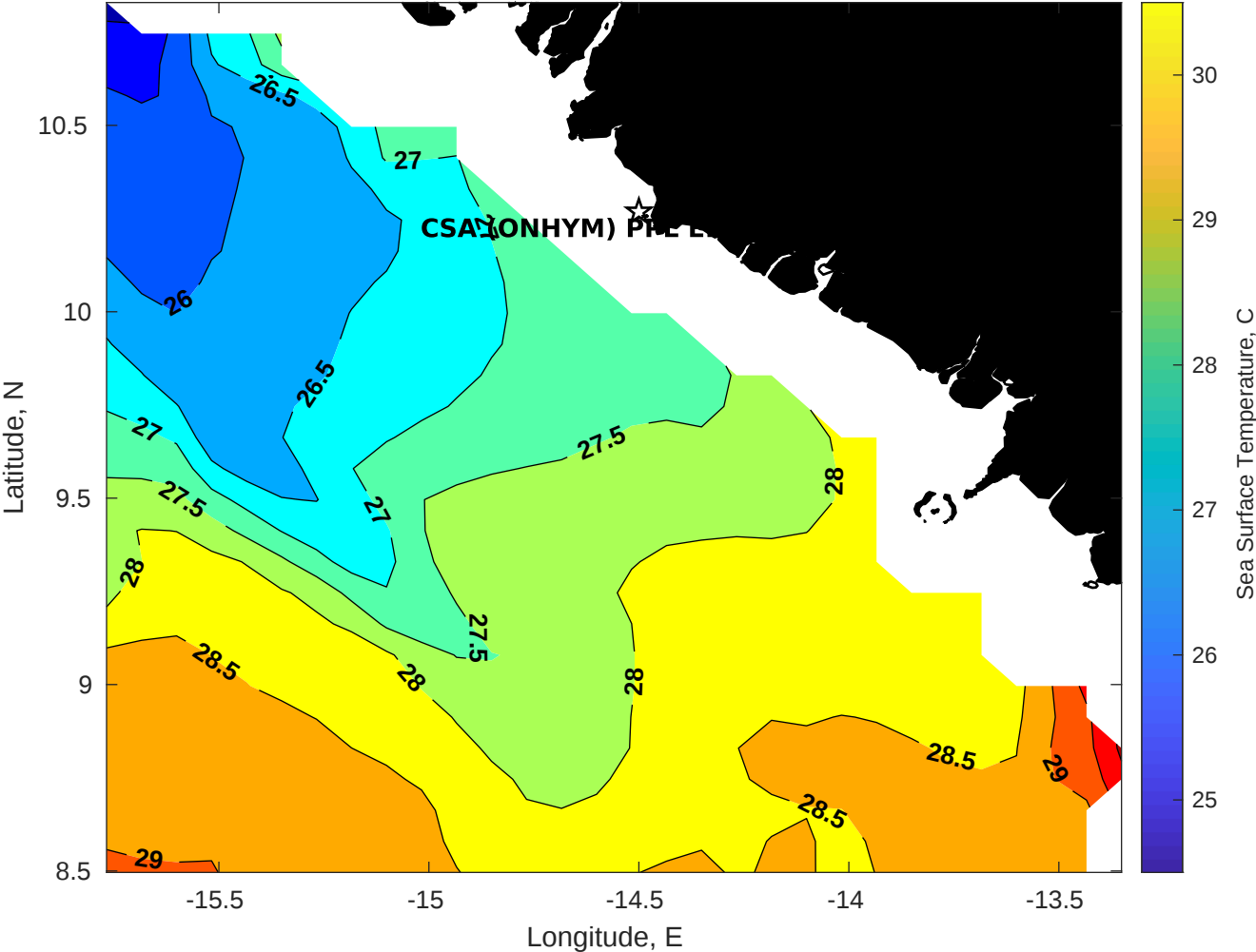
SST for CSA (ONHYM) PPL EBS - Guinea at 15-May-2025 00:00:00
