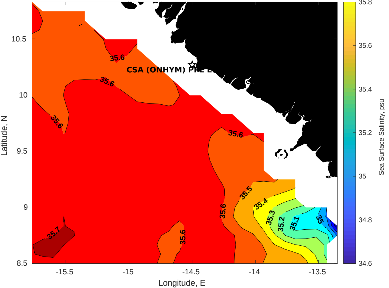
Surface Salinity for CSA (ONHYM) PPL EBS - Guinea at 15-May-2025 00:00:00
