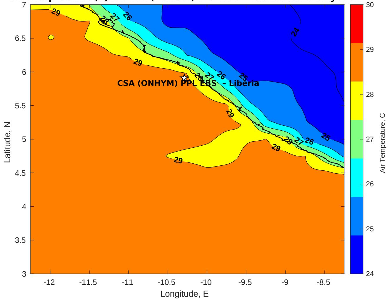
Air Temperature (C) for CSA (ONHYM) PPL EBS - Liberia at 16-May-2025
