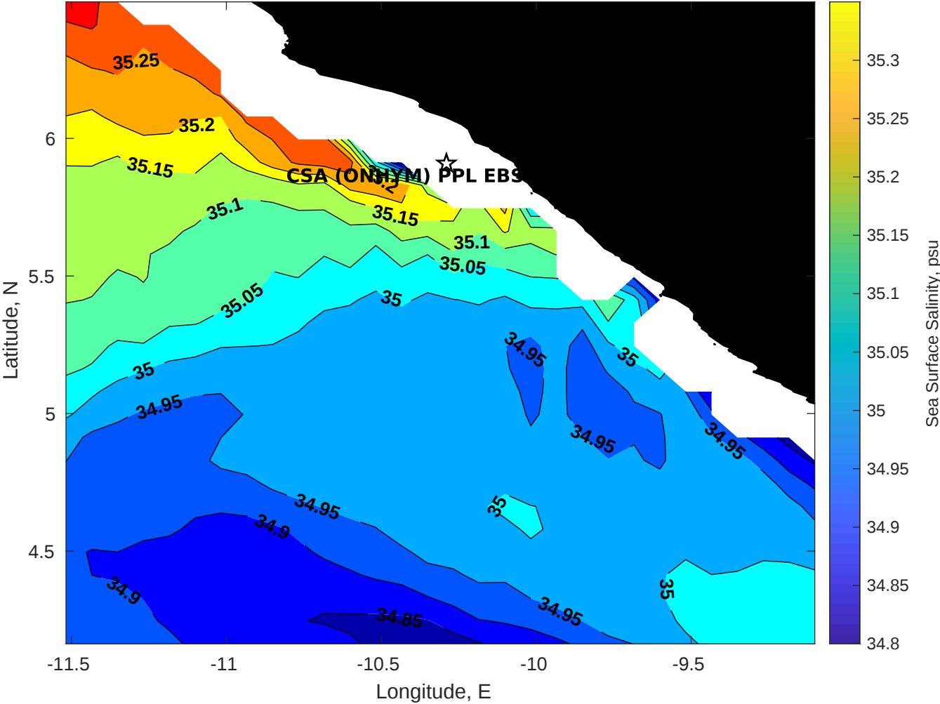
Surface Salinity for CSA (ONHYM) PPL EBS - Liberia at 15-May-2025 00:00:00
