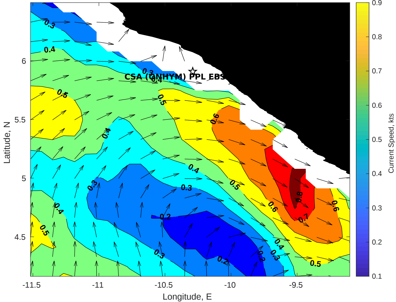
Surface Currents for CSA (ONHYM) PPL EBS - Liberia at 15-May-2025 00:00:00
