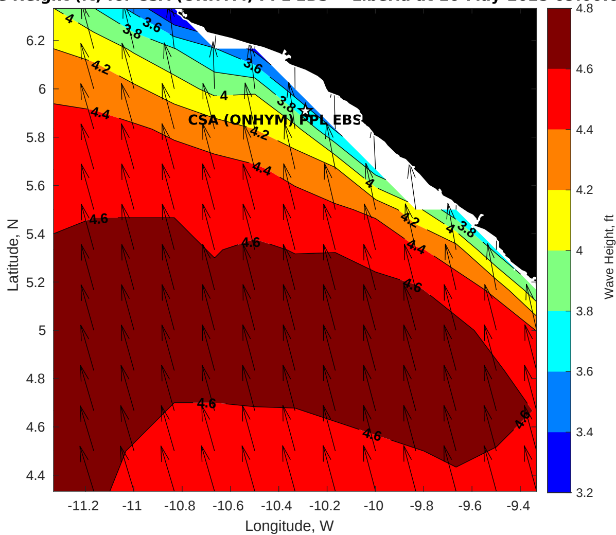
Wave Height (ft) for CSA (ONHYM) PPL EBS - Liberia at 16-May-2025 09:00:00
