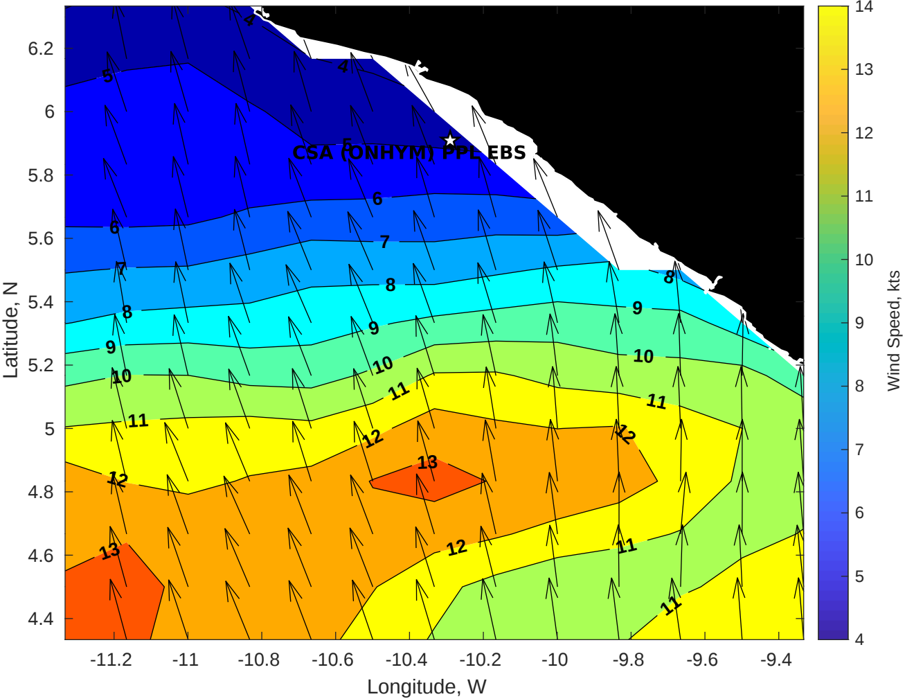
Winds (kts) for CSA (ONHYM) PPL EBS - Liberia at 16-May-2025 09:00:00
