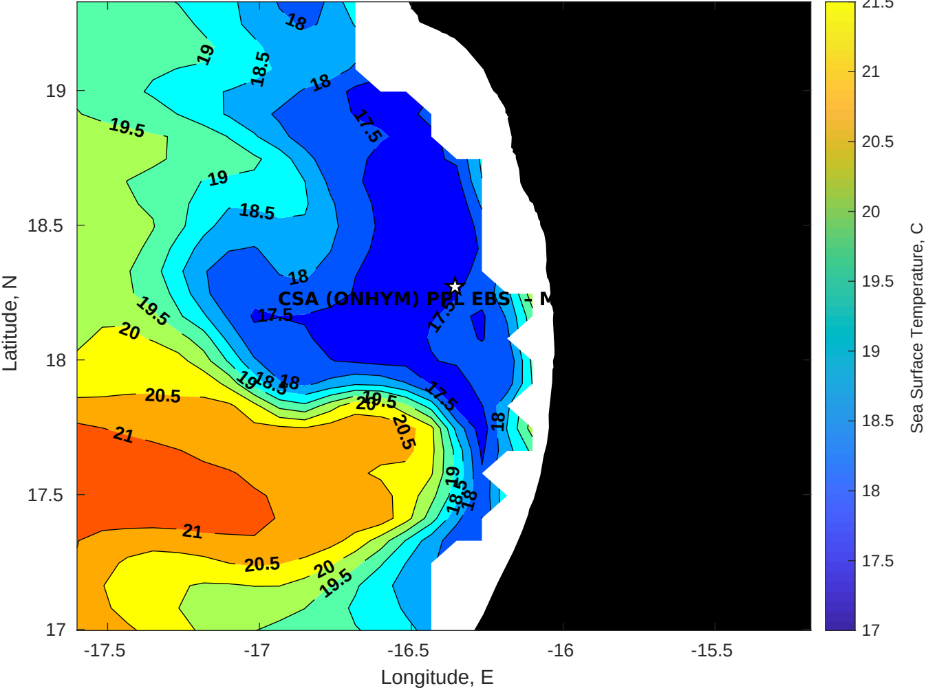
SST for CSA (ONHYM) PPL EBS - Mauritania at 15-May-2025 00:00:00
