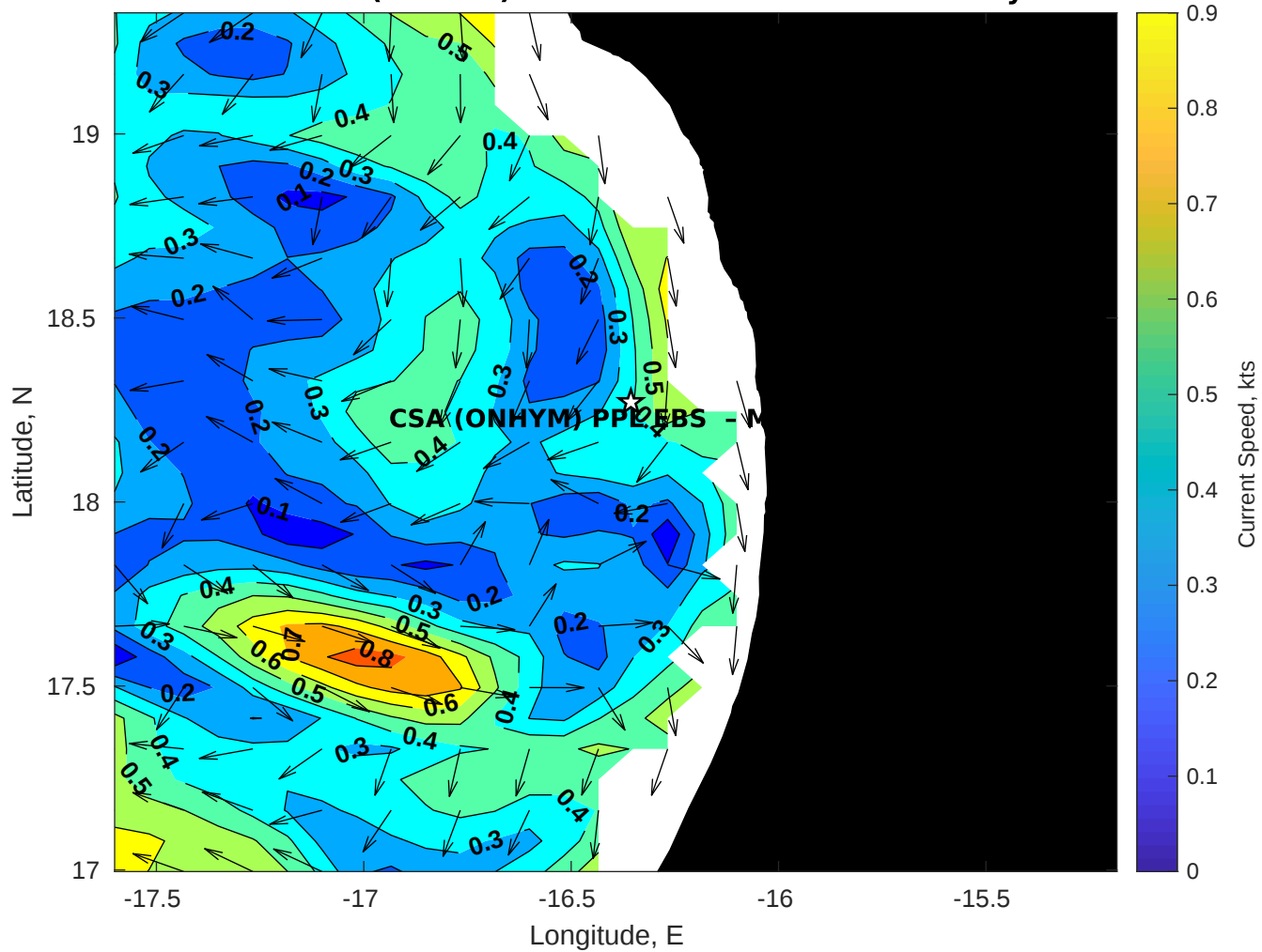
Surface Currents for CSA (ONHYM) PPL EBS - Mauritania at 15-May-2025 00:00:00
