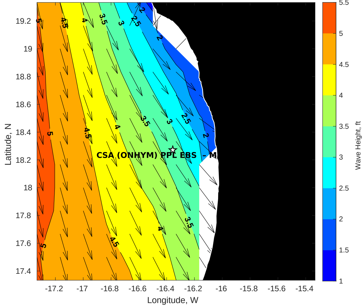
Wave Height (ft) for CSA (ONHYM) PPL EBS - Mauritania at 16-May-2025 09:00:00
