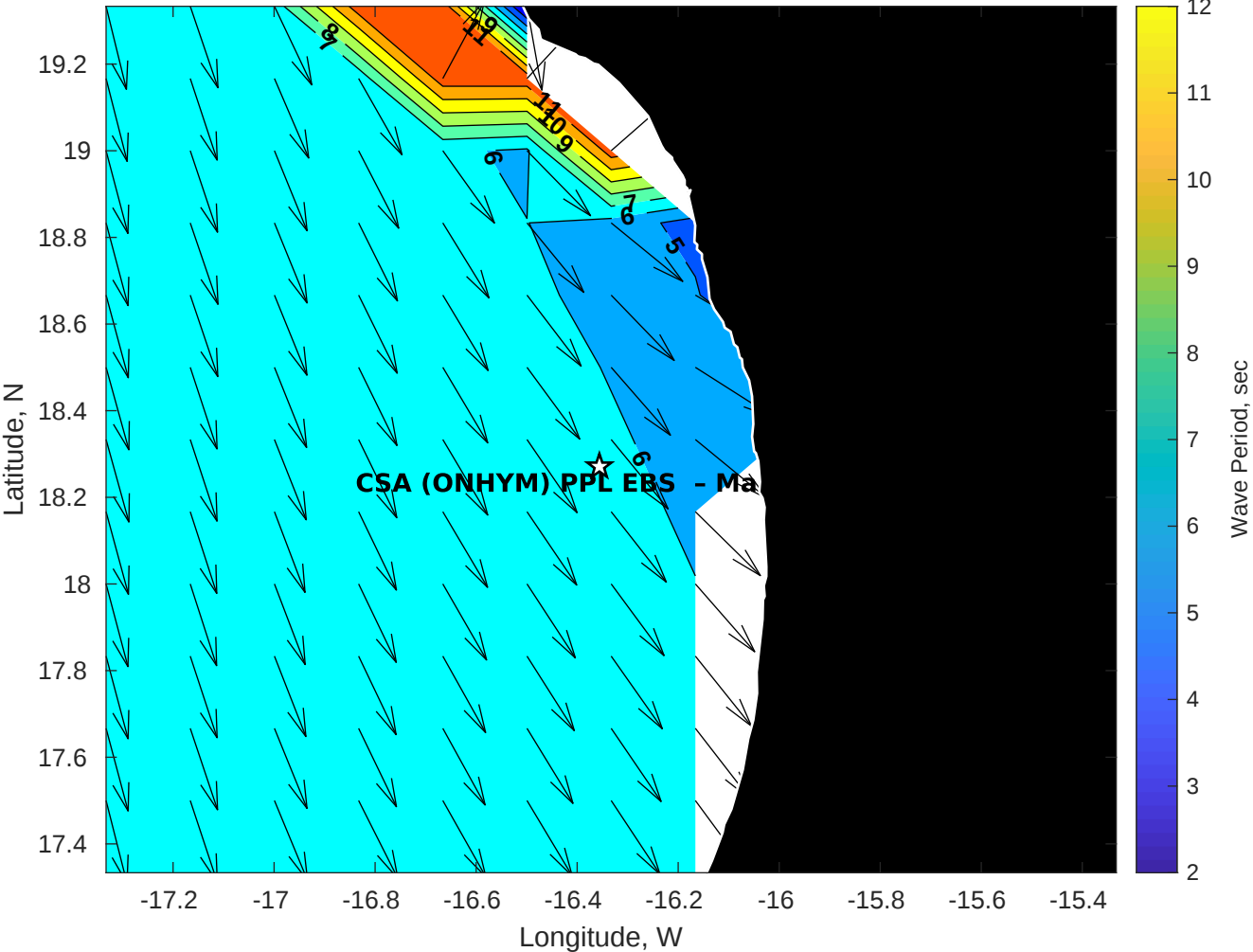
Wave Period (sec) for CSA (ONHYM) PPL EBS - Mauritania at 16-May-2025 09:00:00
