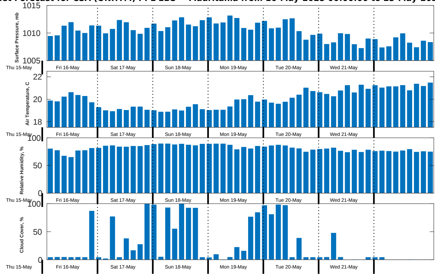
Met Forecast for CSA (ONHYM) PPL EBS - Mauritania from 16-May-2025 00:00:00 to 23-May-2025 00:00:00
