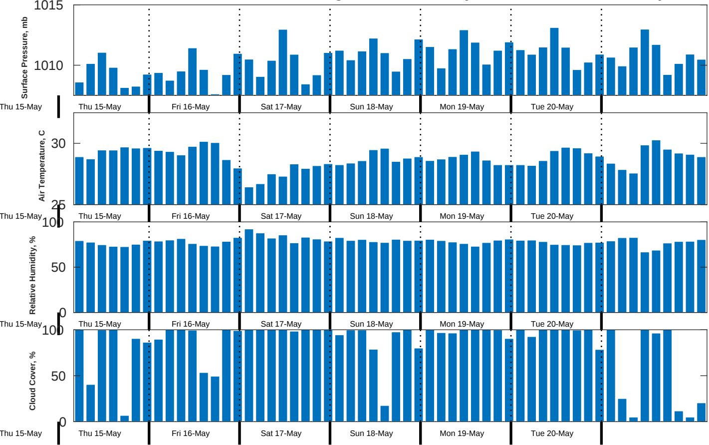
Met Forecast for CSA (ONHYM) PPL EBS - Nigeria from 16-May-2025 00:00:00 to 23-May-2025 00:00:00
