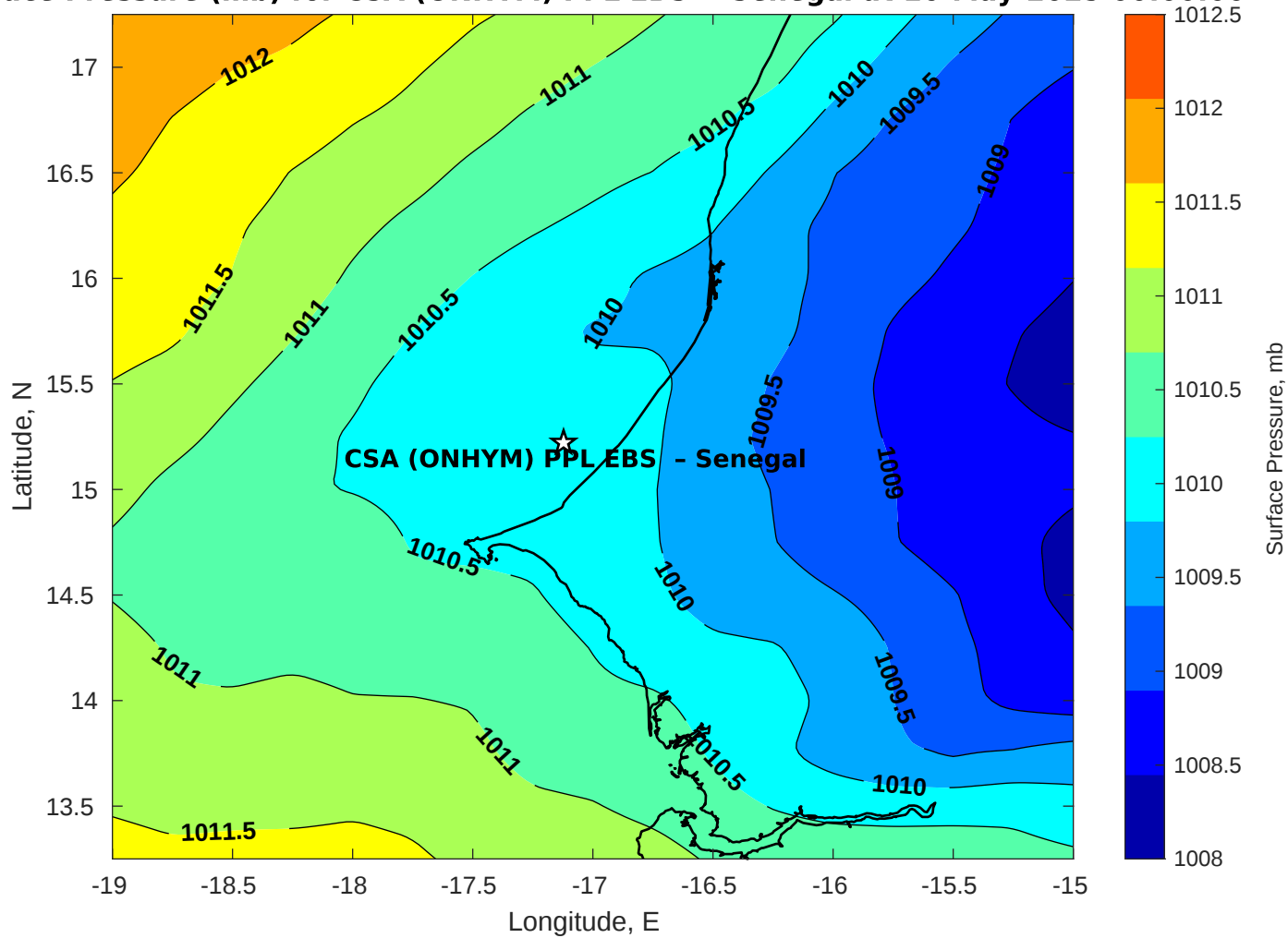
Surface Pressure (mb) for CSA (ONHYM) PPL EBS - Senegal at 16-May-2025 00:00:00
