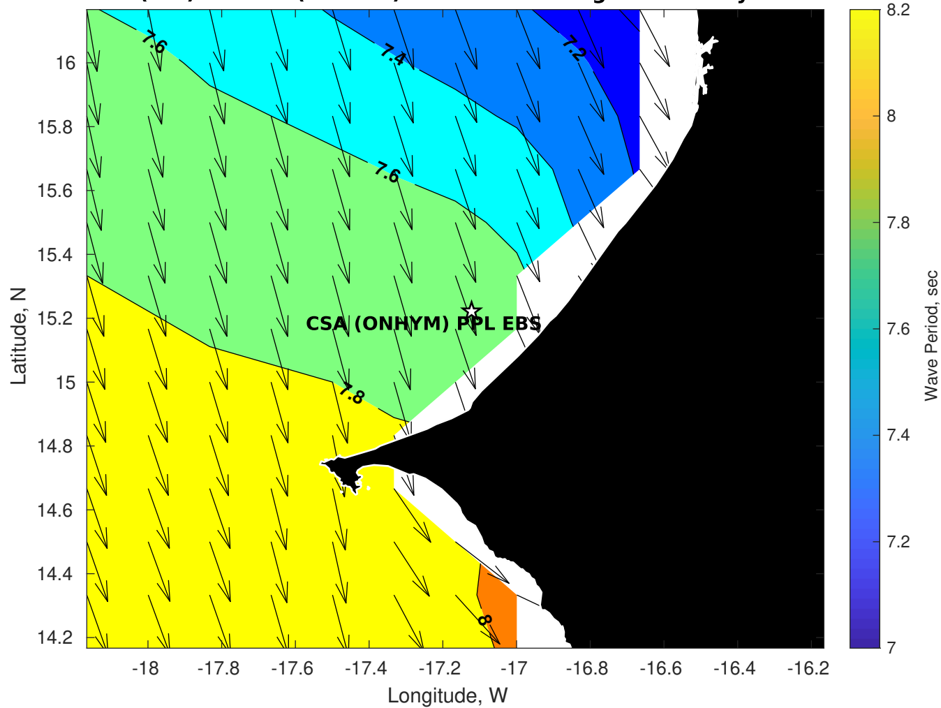
Wave Period (sec) for CSA (ONHYM) PPL EBS - Senegal at 16-May-2025 09:00:00
