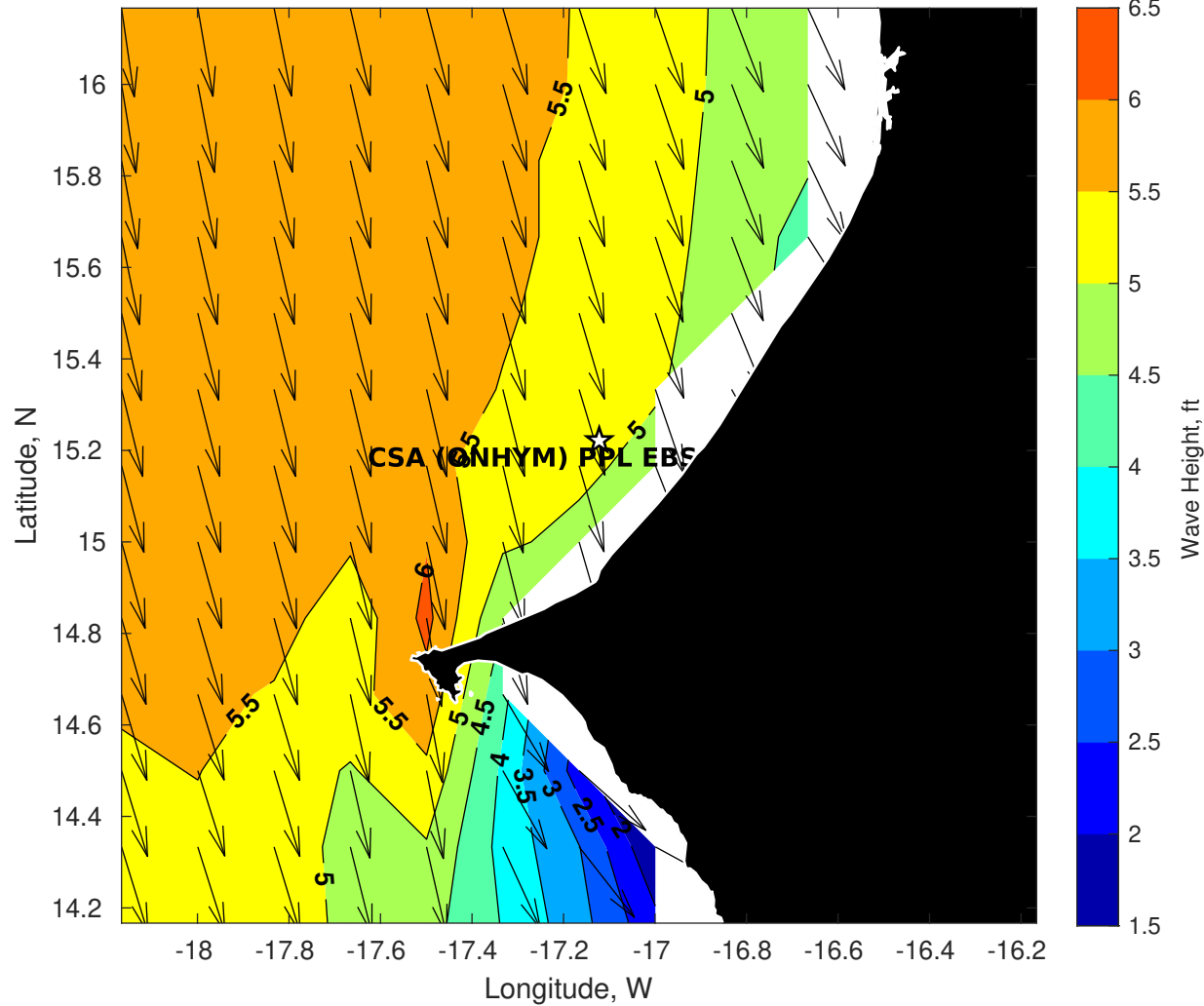
Wave Height (ft) for CSA (ONHYM) PPL EBS - Senegal at 16-May-2025 09:00:00
