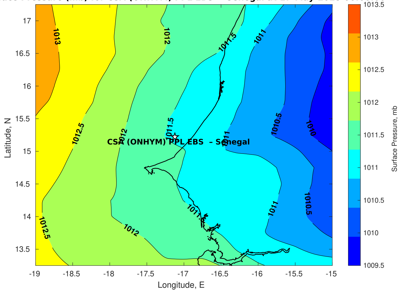
Surface Pressure (mb) for CSA (ONHYM) PPL EBS - Senegal at 17-May-2025 00:00:00
