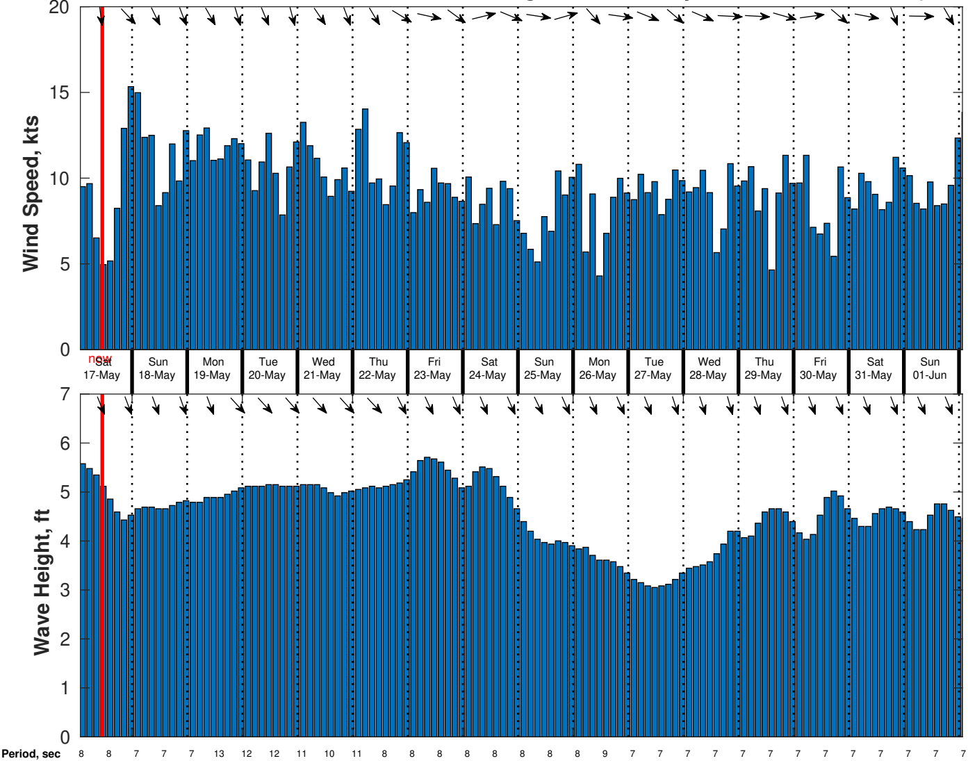
Wind & Wave Forecast for CSA (ONHYM) PPL EBS - Senegal from 16-May-2025 01:00:00 to 01-Jun-2025 01:00:00
