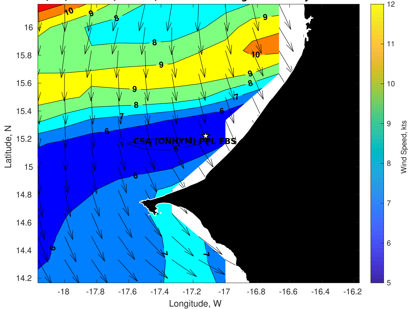
Winds (kts) for CSA (ONHYM) PPL EBS - Senegal at 16-May-2025 09:00:00
