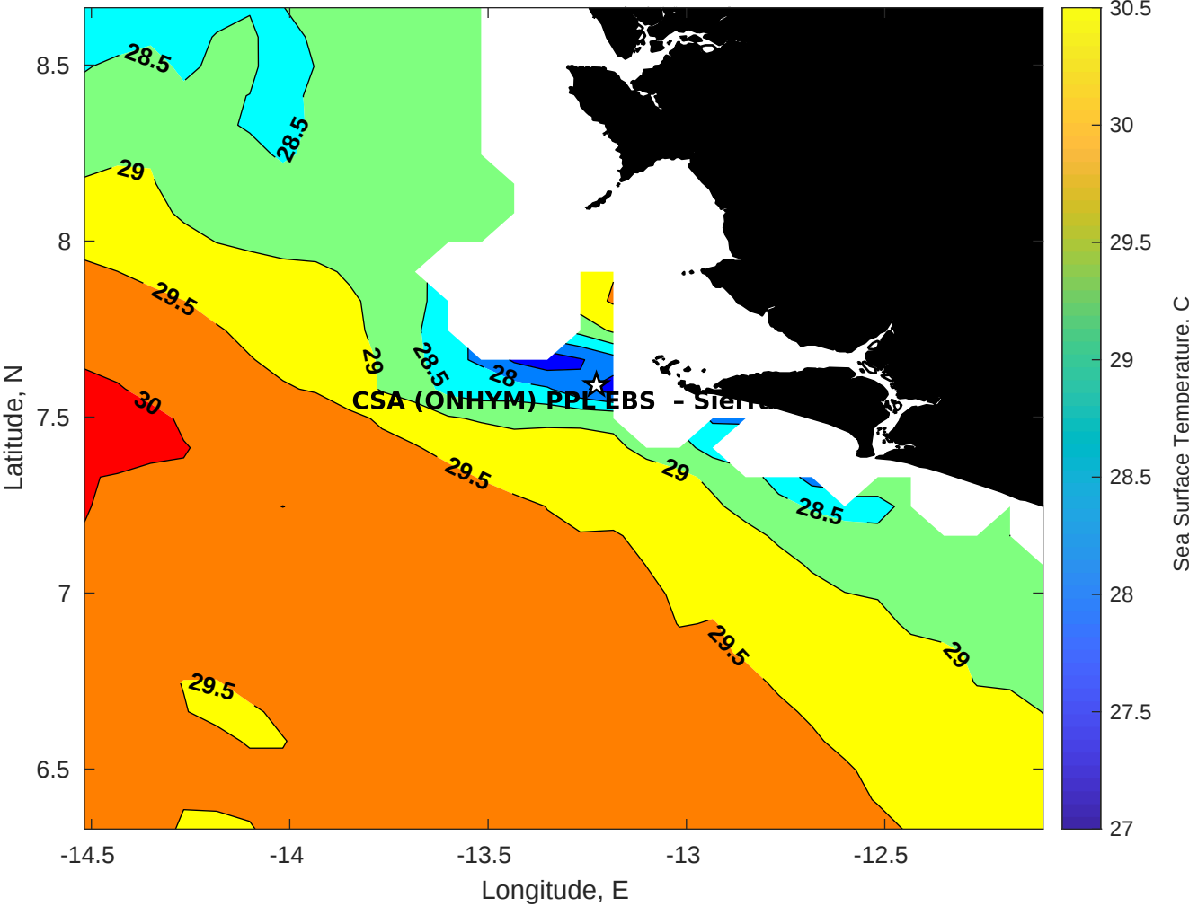
SST for CSA (ONHYM) PPL EBS - Sierra Leone at 15-May-2025 00:00:00
