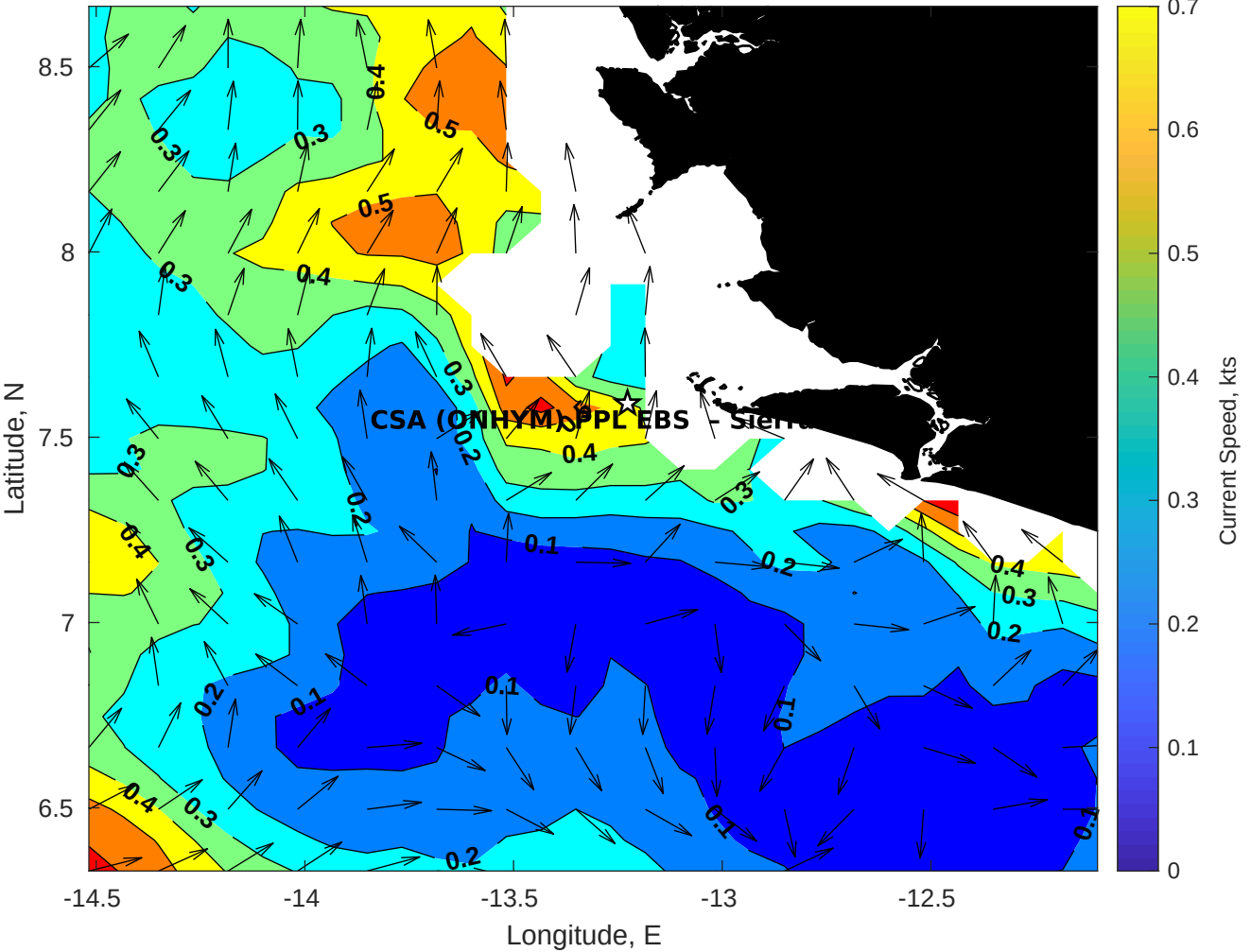
Surface Currents for CSA (ONHYM) PPL EBS - Sierra Leone at 15-May-2025 00:00:00
