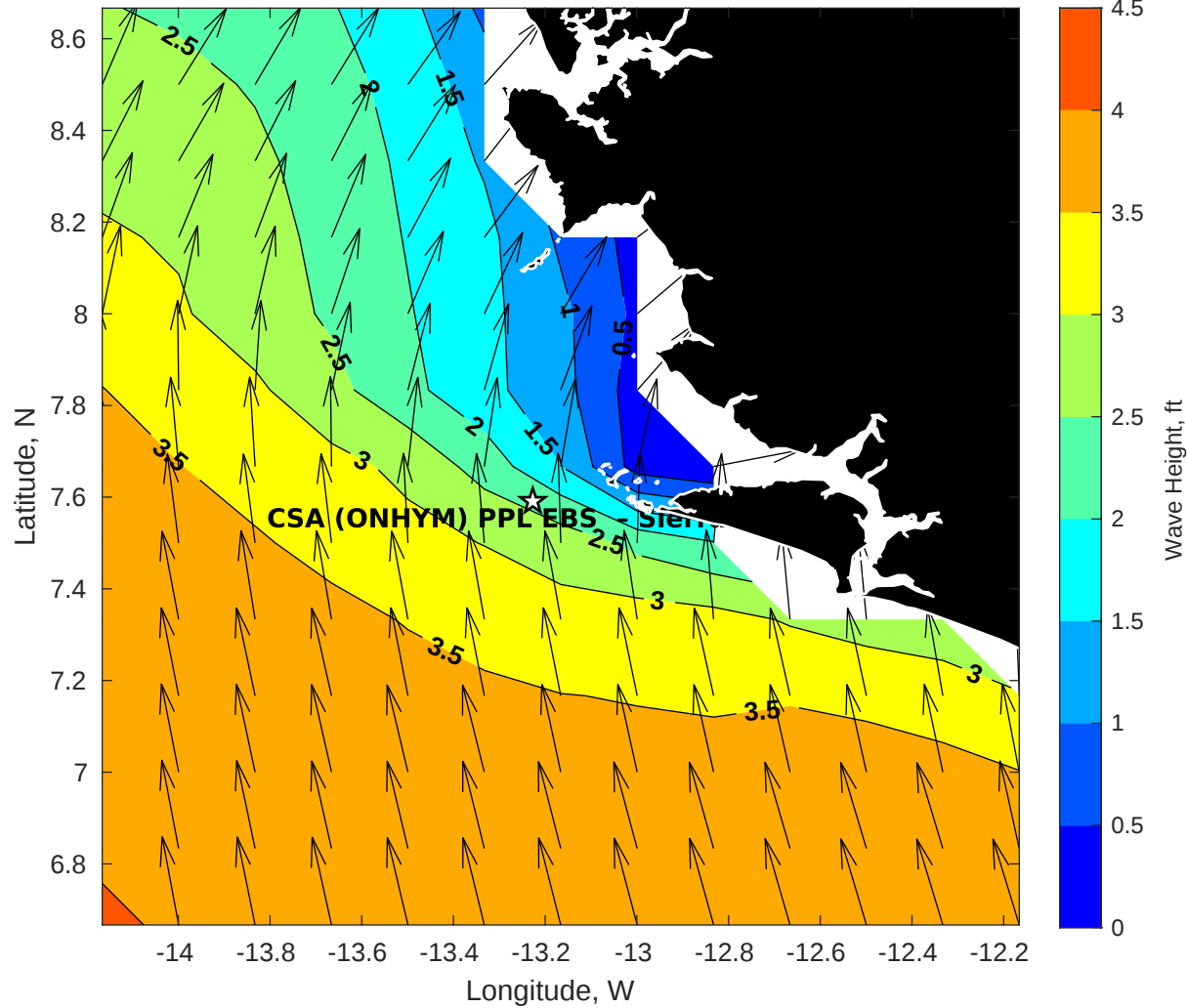
Wave Height (ft) for CSA (ONHYM) PPL EBS - Sierra Leone at 16-May-2025 09:00:00
