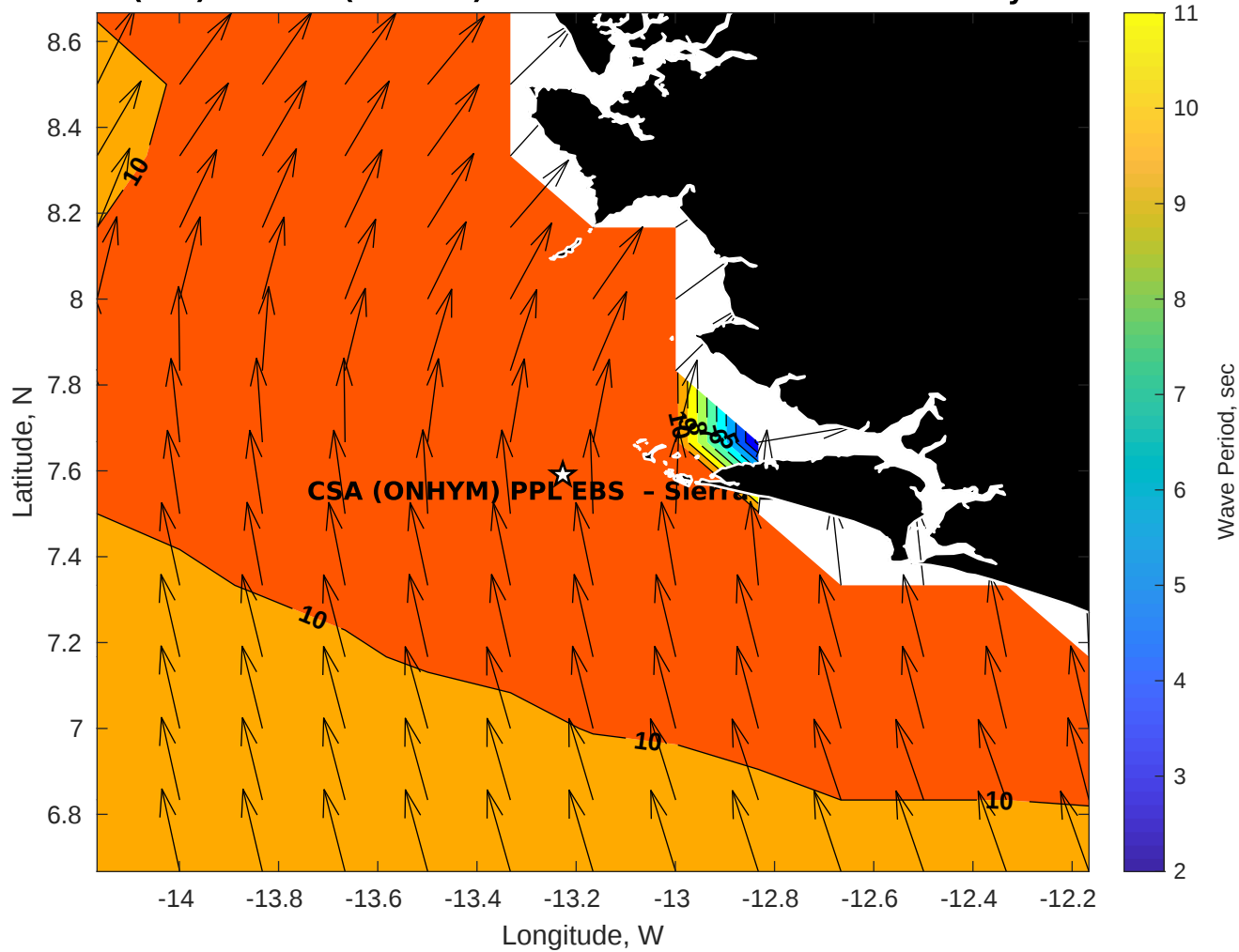
Wave Period (sec) for CSA (ONHYM) PPL EBS - Sierra Leone at 16-May-2025 09:00:00
