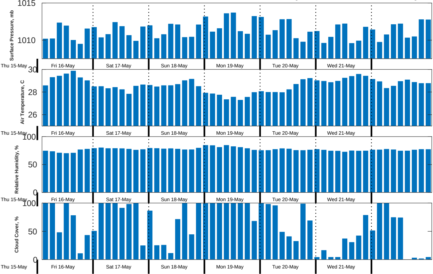
Met Forecast for CSA (ONHYM) PPL EBS - Sierra Leone from 16-May-2025 00:00:00 to 23-May-2025 00:00:00
