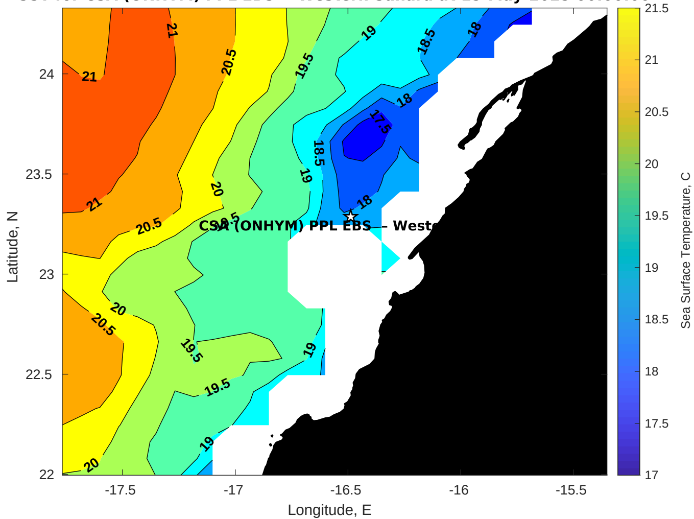
SST for CSA (ONHYM) PPL EBS - Western Sahara at 15-May-2025 00:00:00
