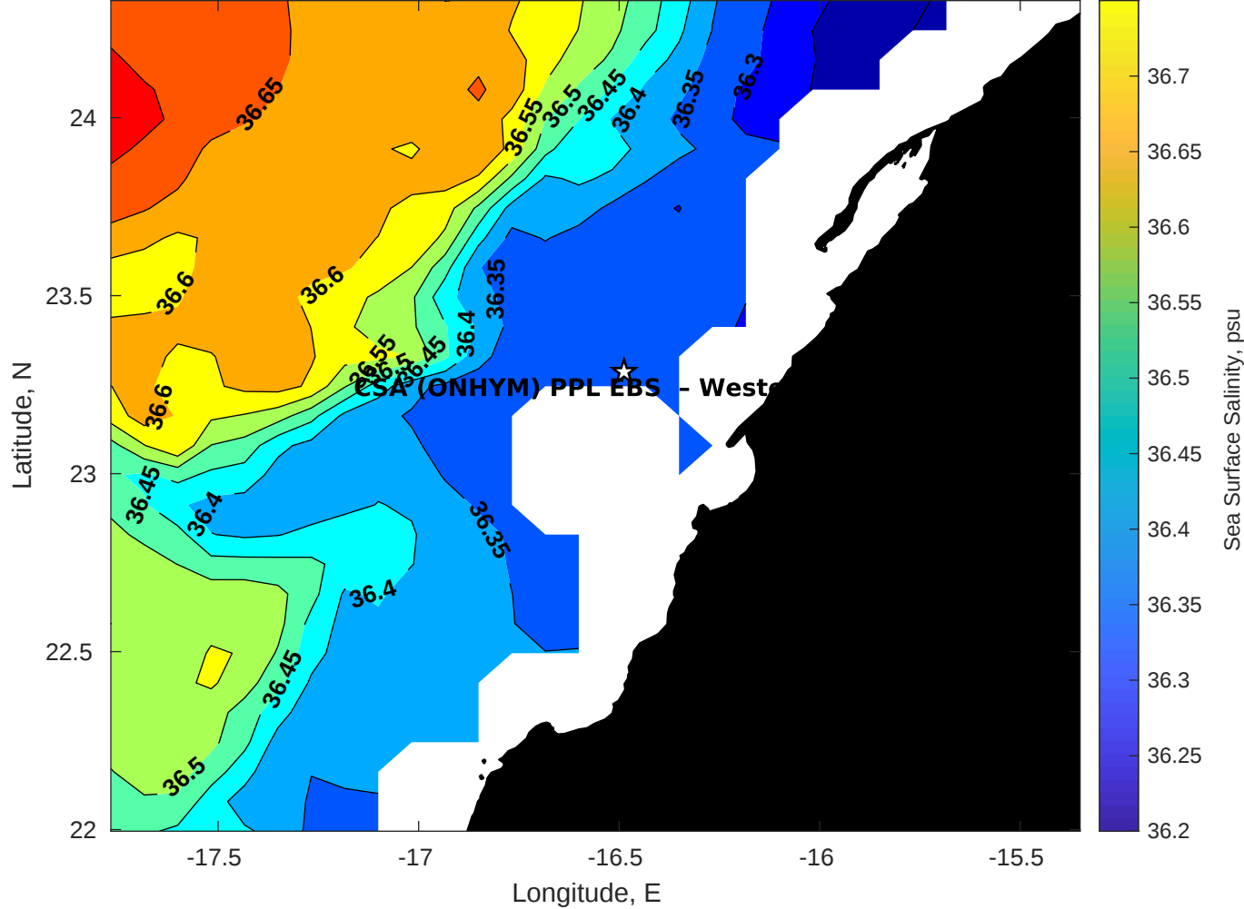
Surface Salinity for CSA (ONHYM) PPL EBS - Western Sahara at 15-May-2025 00:00:00
