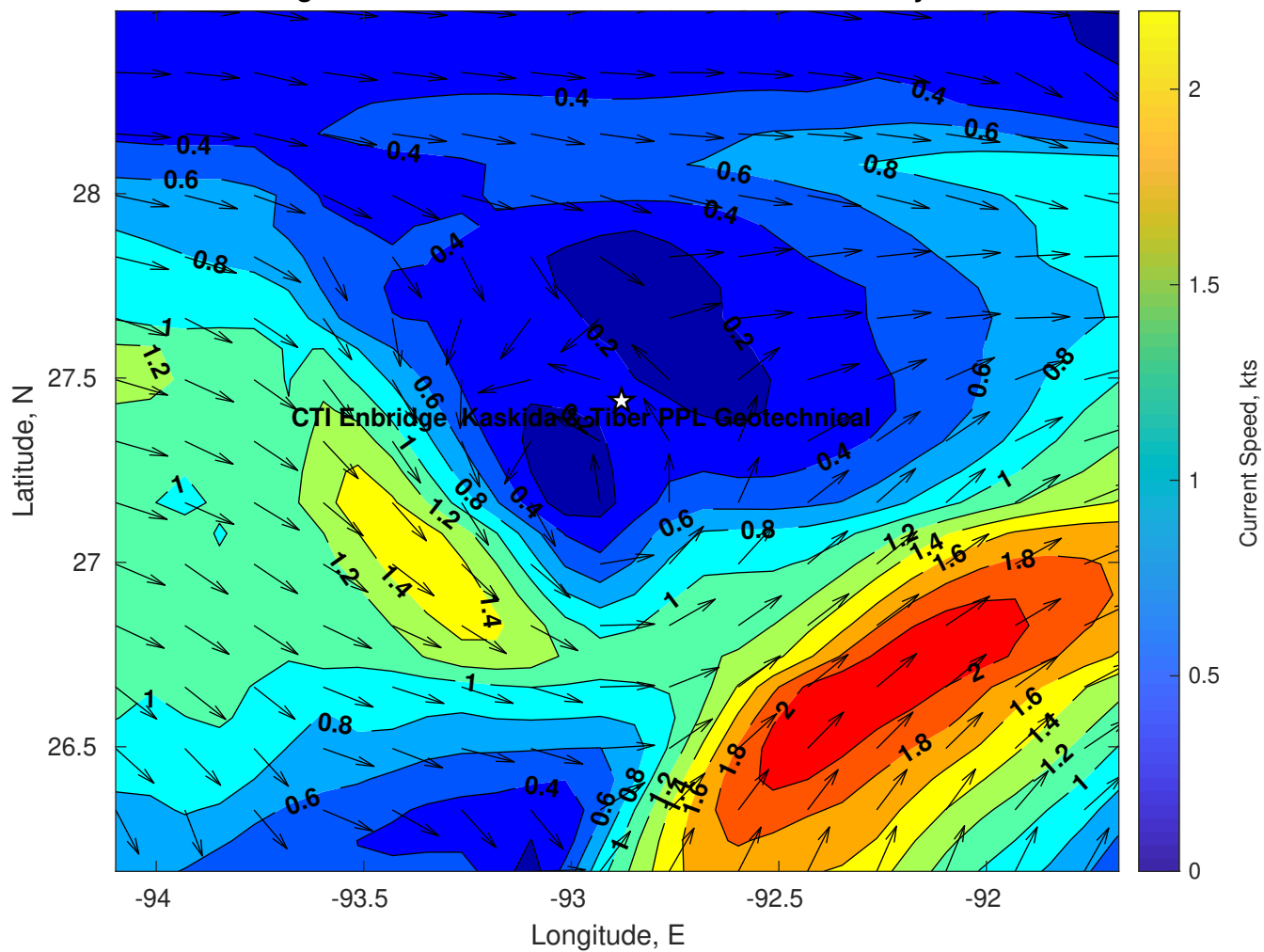
Surface Currents for CTI Enbridge Kaskida & Tiber PPL Geotechnical at 15-May-2025 00:00:00
