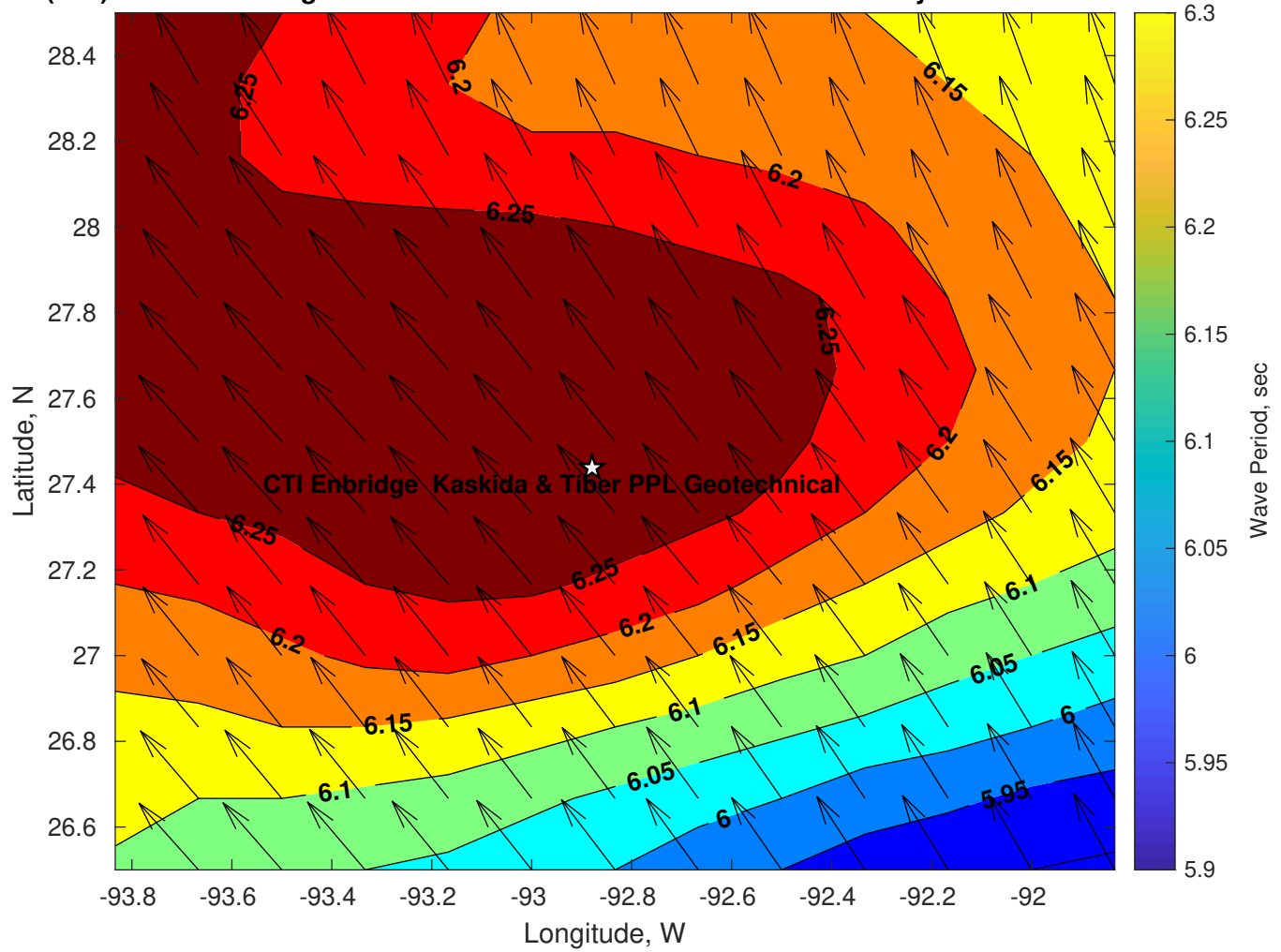
Wave Period (sec) for CTI Enbridge Kaskida & Tiber PPL Geotechnical at 16-May-2025 09:00:00
