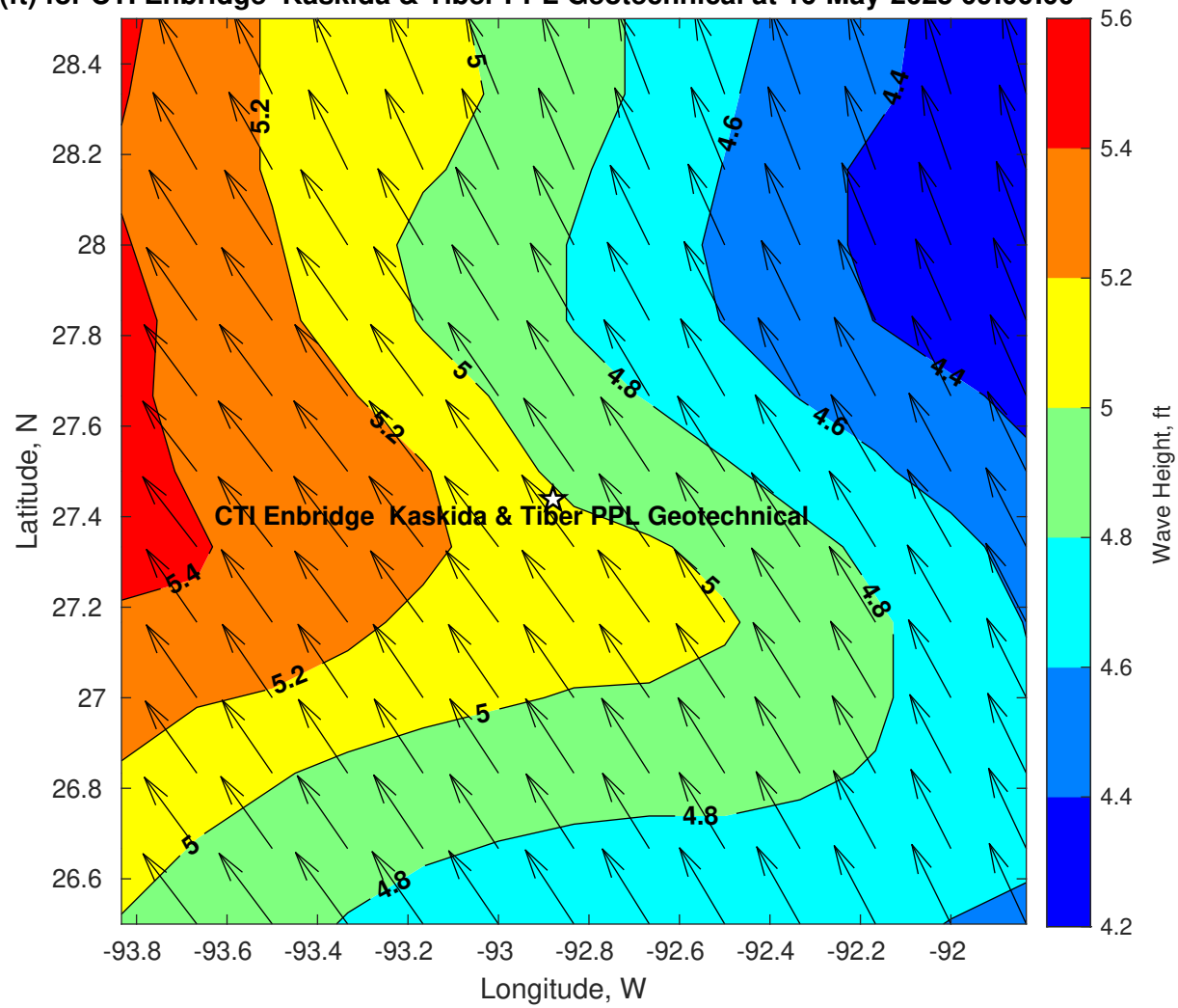
Wave Height (ft) for CTI Enbridge Kaskida & Tiber PPL Geotechnical at 16-May-2025 09:00:00
