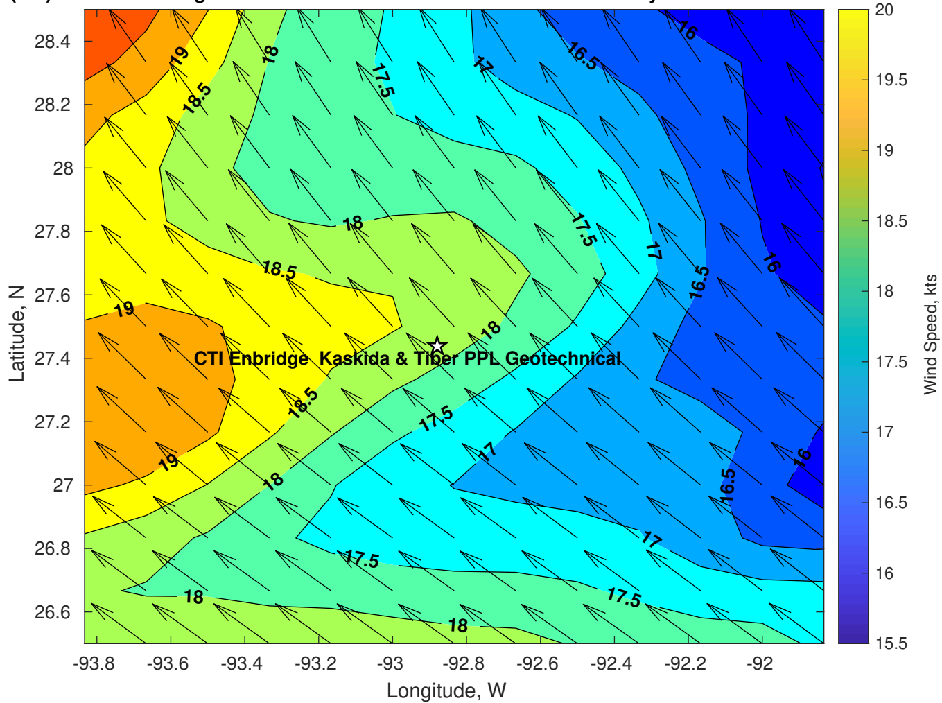
Winds (kts) for CTI Enbridge Kaskida & Tiber PPL Geotechnical at 16-May-2025 09:00:00
