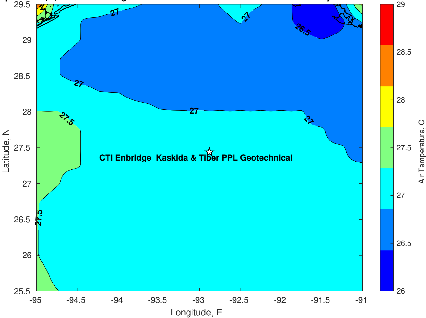
Air Temperature (C) for CTI Enbridge Kaskida & Tiber PPL Geotechnical at 16-May-2025
