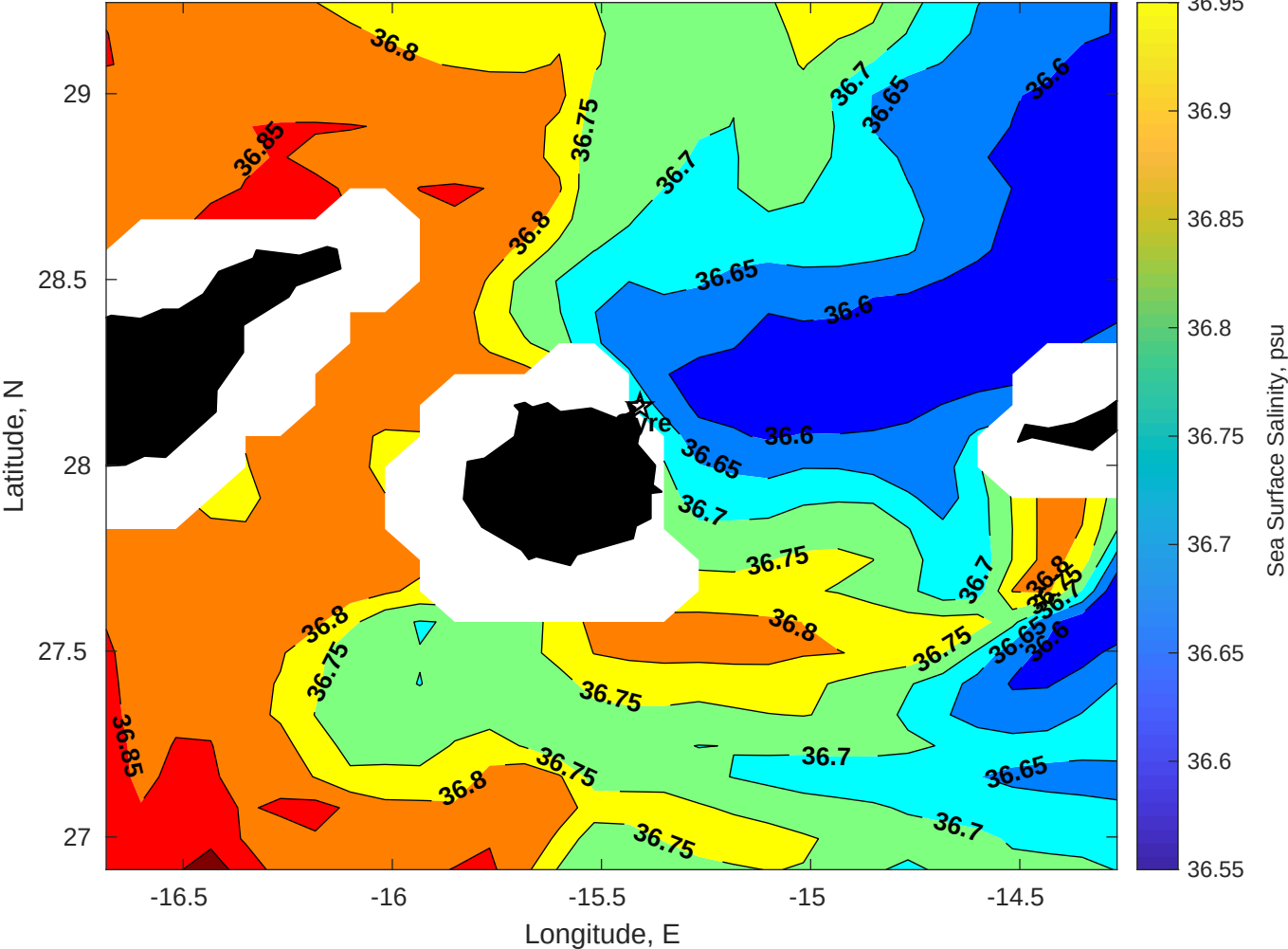
Surface Salinity for Gyre at 15-May-2025 00:00:00
