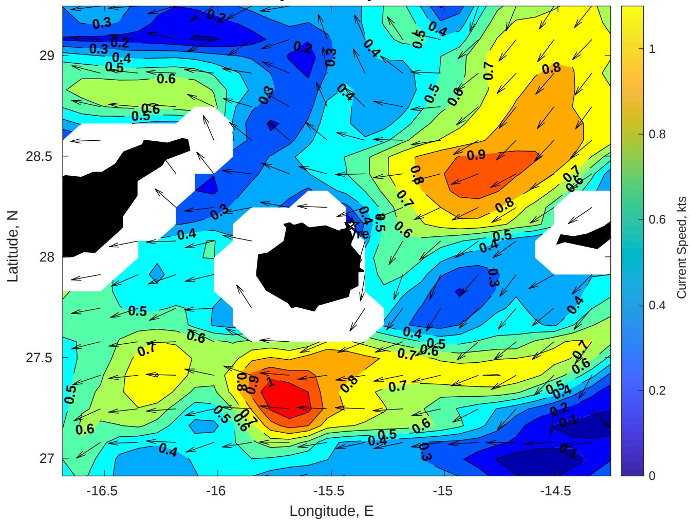
Surface Currents for Gyre at 15-May-2025 00:00:00
