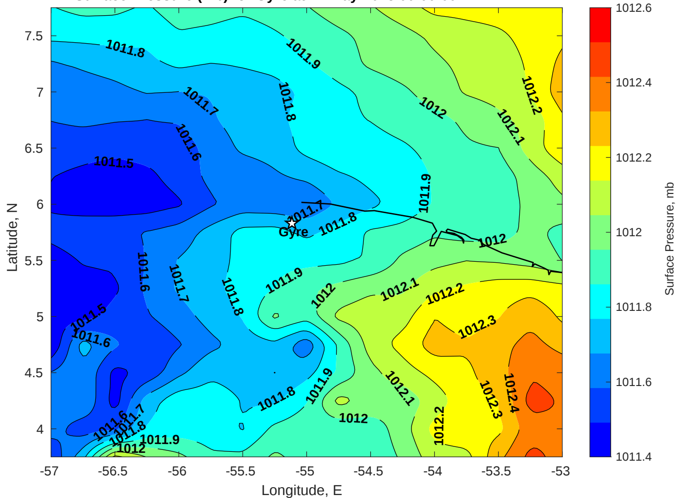
Surface Pressure (mb) for Gyre at 17-May-2025 00:00:00
