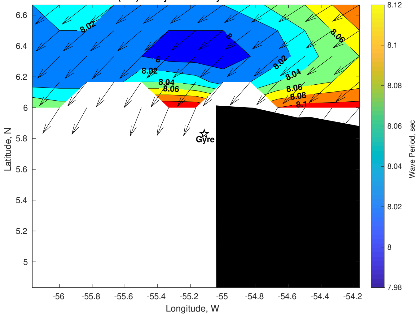
Wave Period (sec) for Gyre at 16-May-2025 09:00:00
