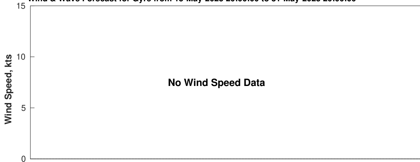
Wind & Wave Forecast for Gyre from 15-May-2025 20:00:00 to 31-May-2025 20:00:00
