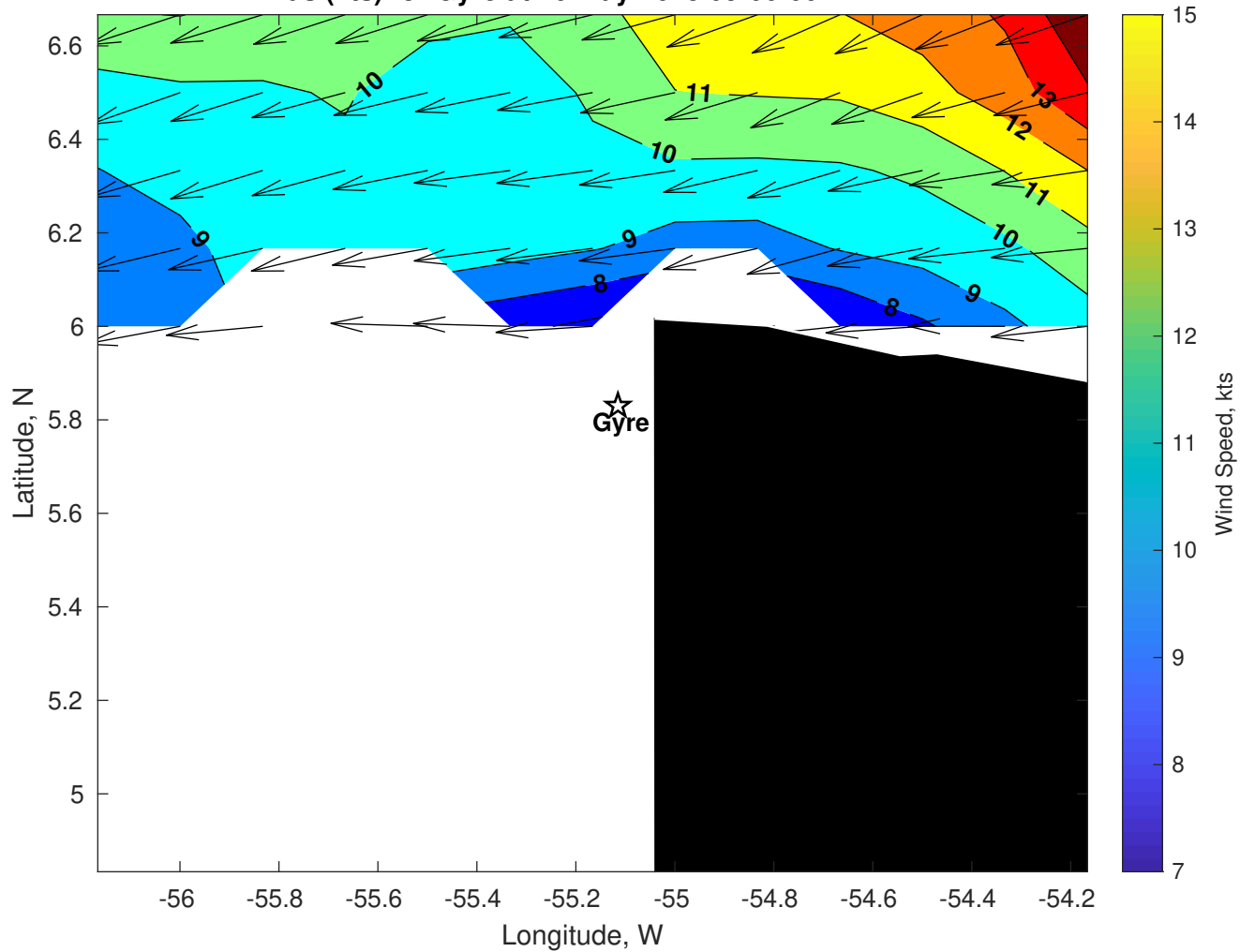
Winds (kts) for Gyre at 16-May-2025 09:00:00
