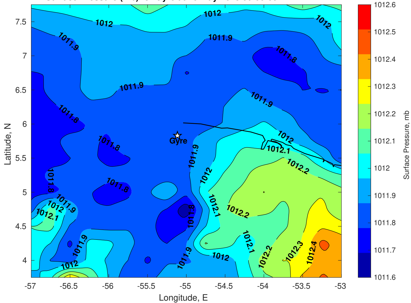
Surface Pressure (mb) for Gyre at 16-May-2025 00:00:00
