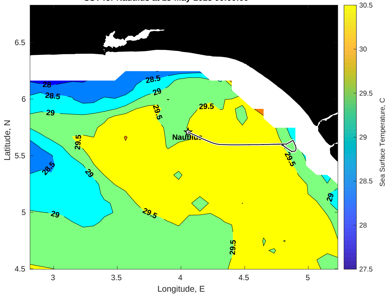
SST for Nautilus at 15-May-2025 00:00:00
