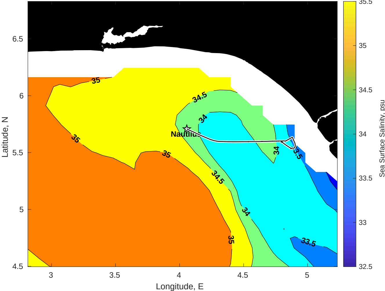
Surface Salinity for Nautilus at 15-May-2025 00:00:00
