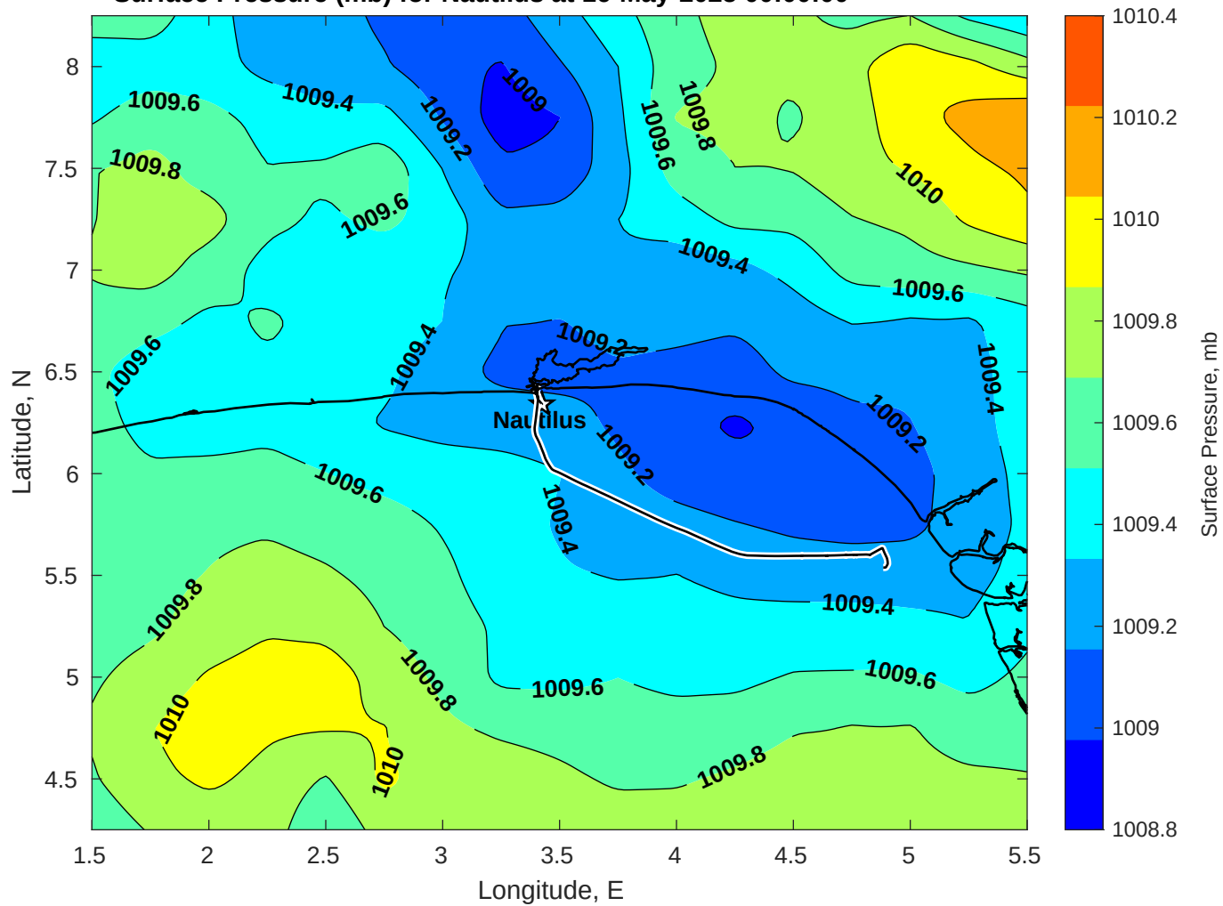
Surface Pressure (mb) for Nautilus at 16-May-2025 00:00:00
