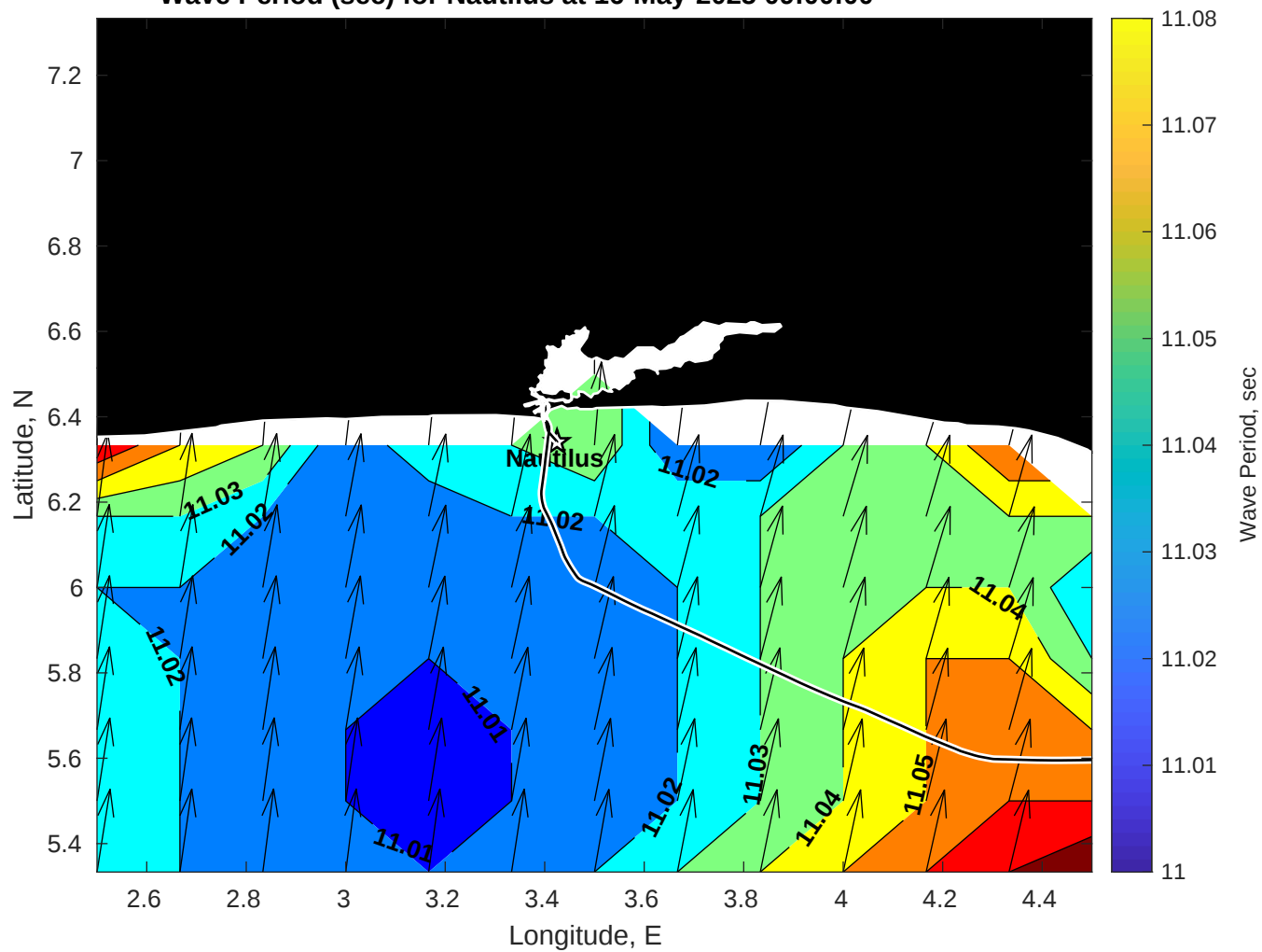
Wave Period (sec) for Nautilus at 16-May-2025 09:00:00
