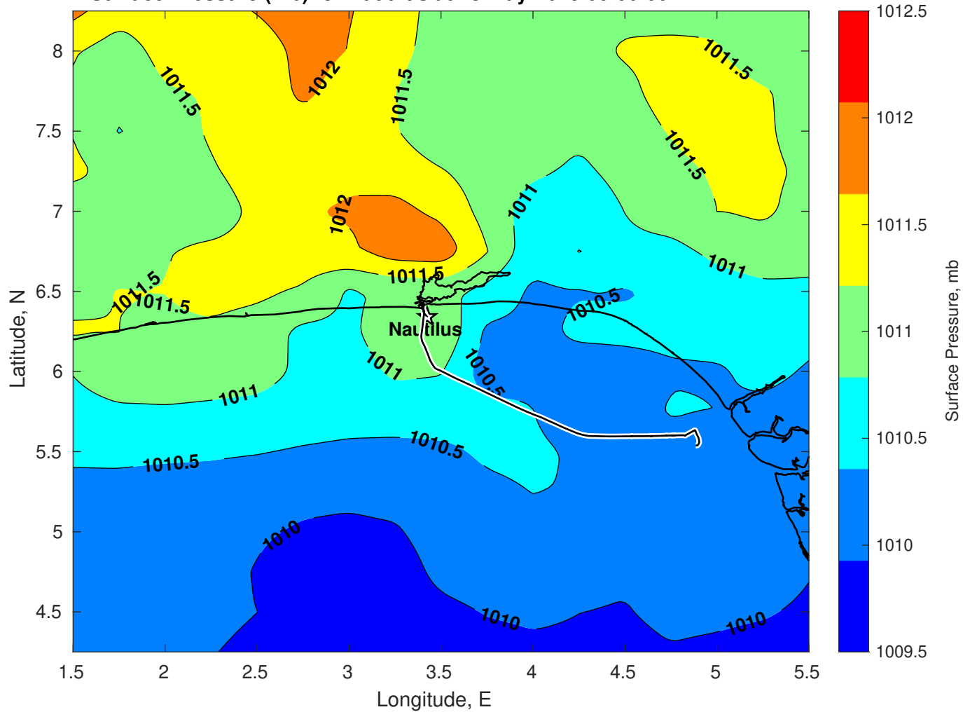
Surface Pressure (mb) for Nautilus at 18-May-2025 00:00:00
