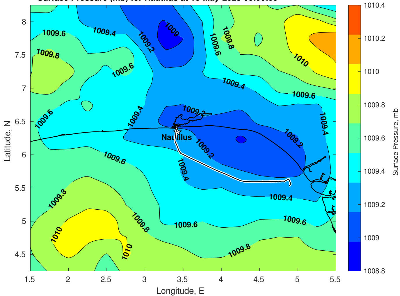
Surface Pressure (mb) for Nautilus at 16-May-2025 00:00:00
