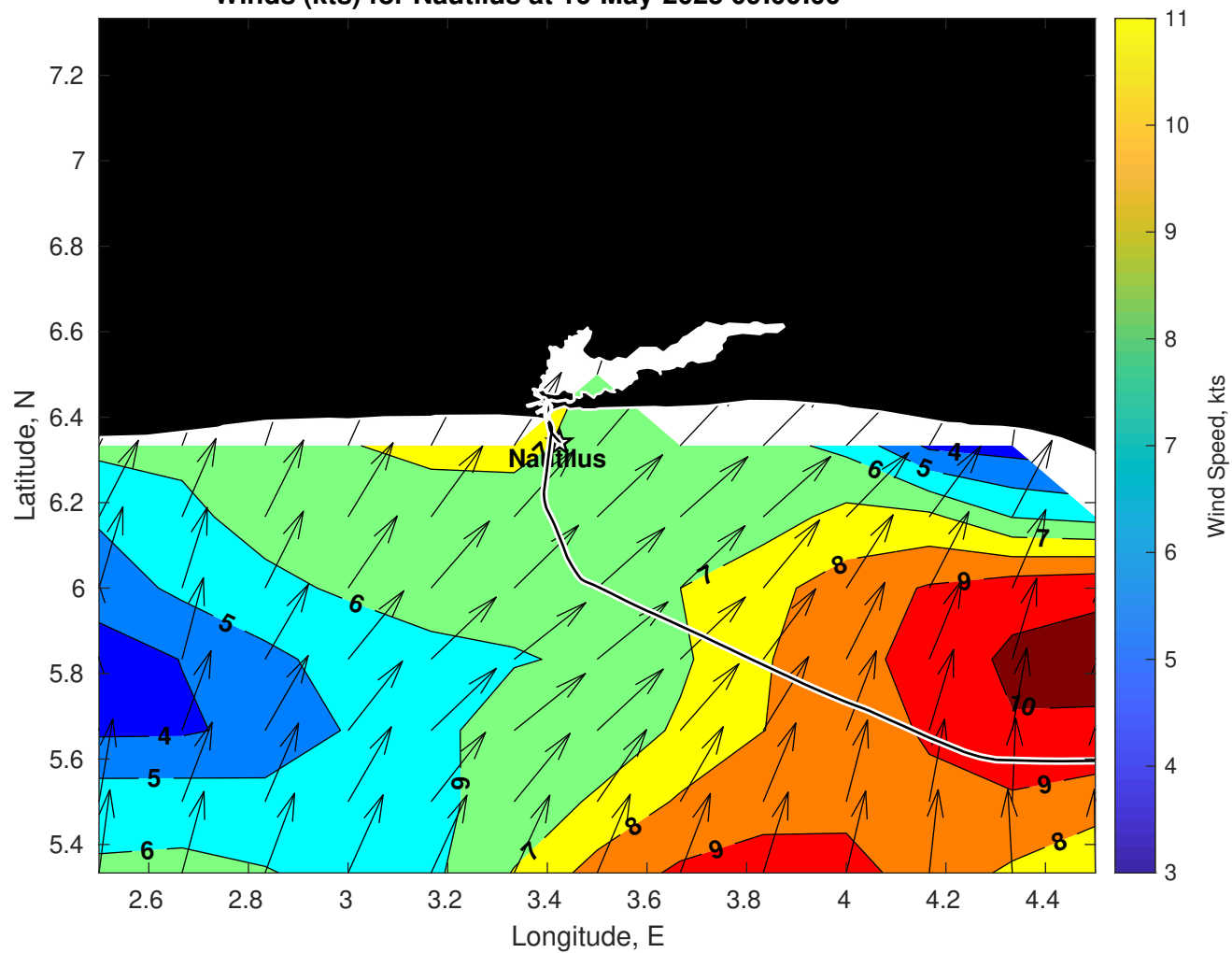
Winds (kts) for Nautilus at 16-May-2025 09:00:00
