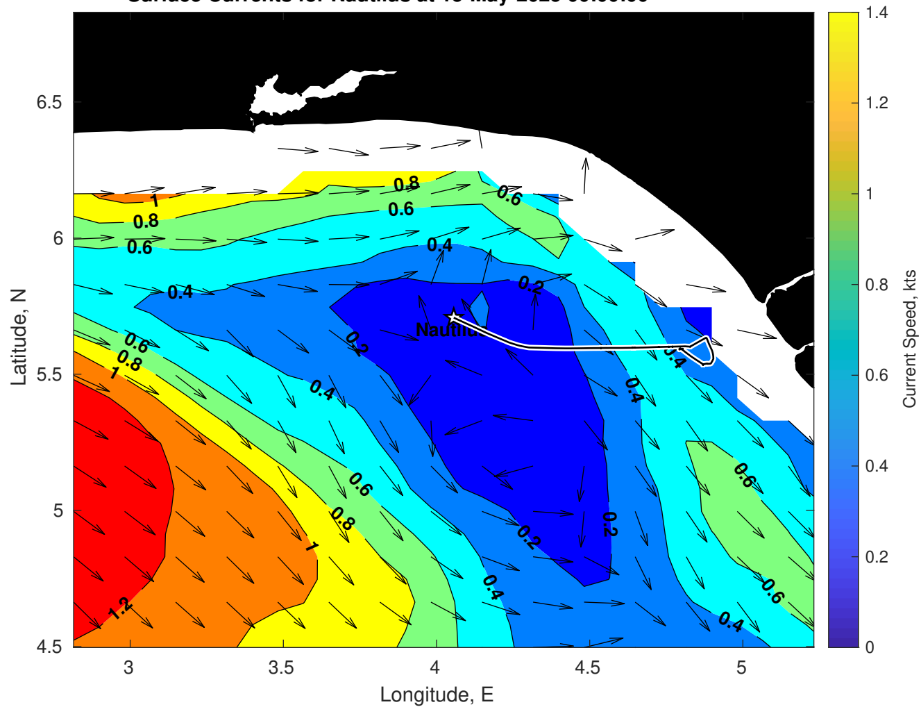
Surface Currents for Nautilus at 15-May-2025 00:00:00
