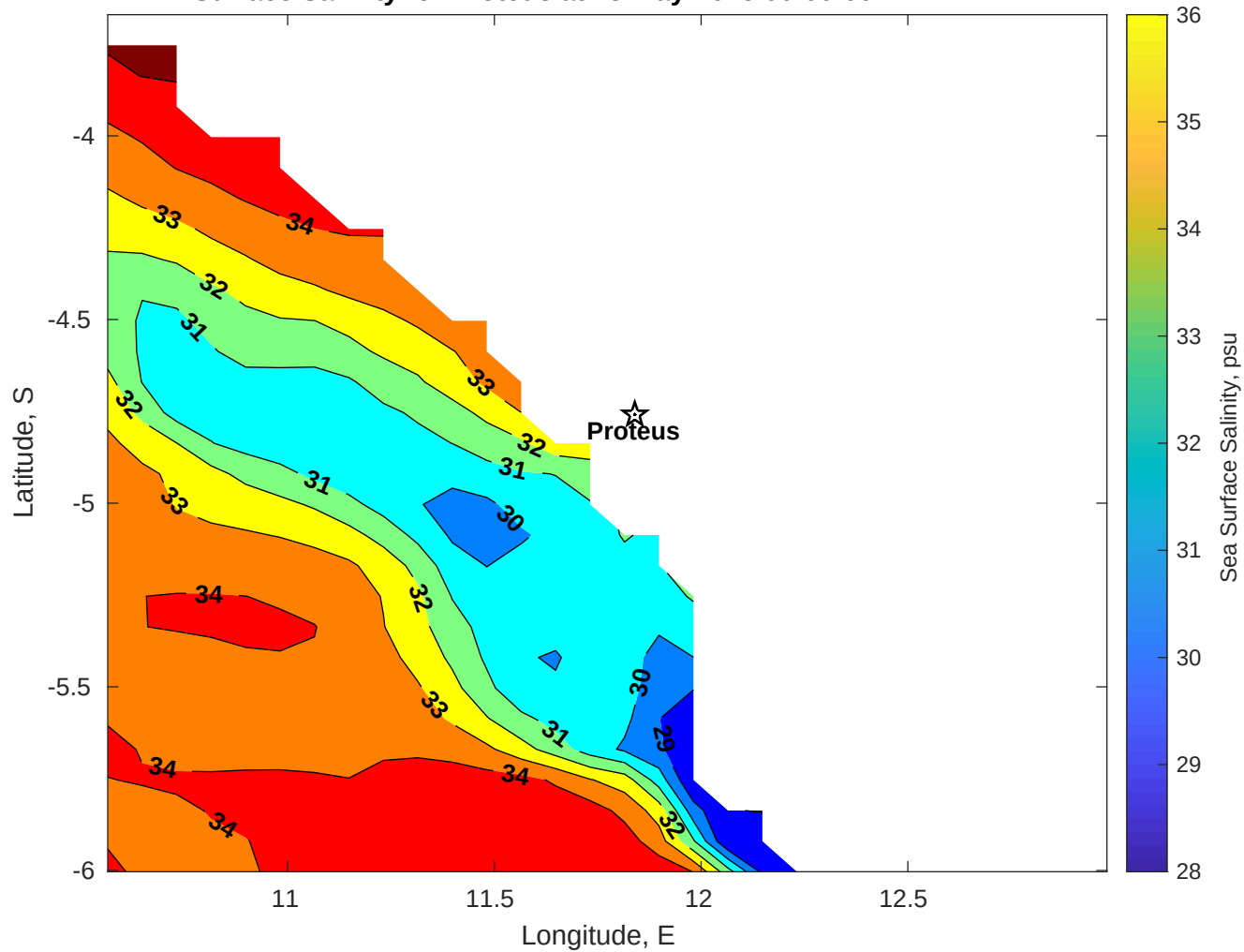
Surface Salinity for Proteus at 15-May-2025 00:00:00
