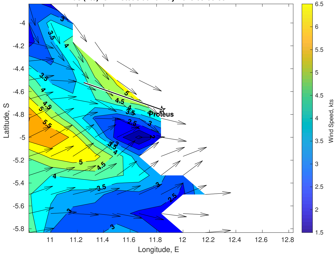
Winds (kts) for Proteus at 16-May-2025 09:00:00
