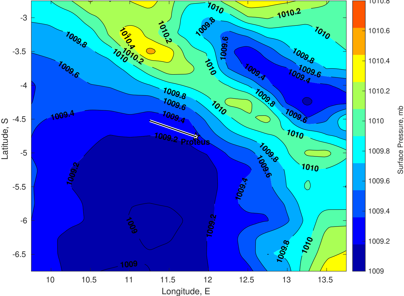
Surface Pressure (mb) for Proteus at 18-May-2025 00:00:00
