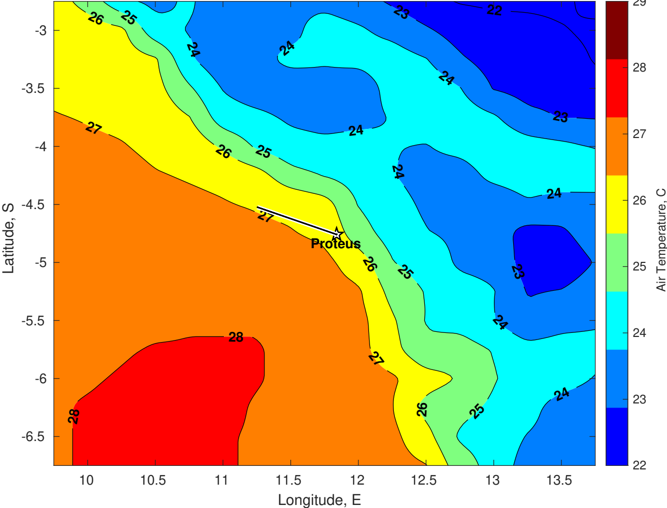
Air Temperature (C) for Proteus at 16-May-2025
