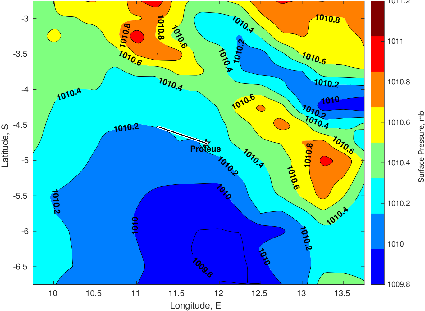
Surface Pressure (mb) for Proteus at 16-May-2025 00:00:00
