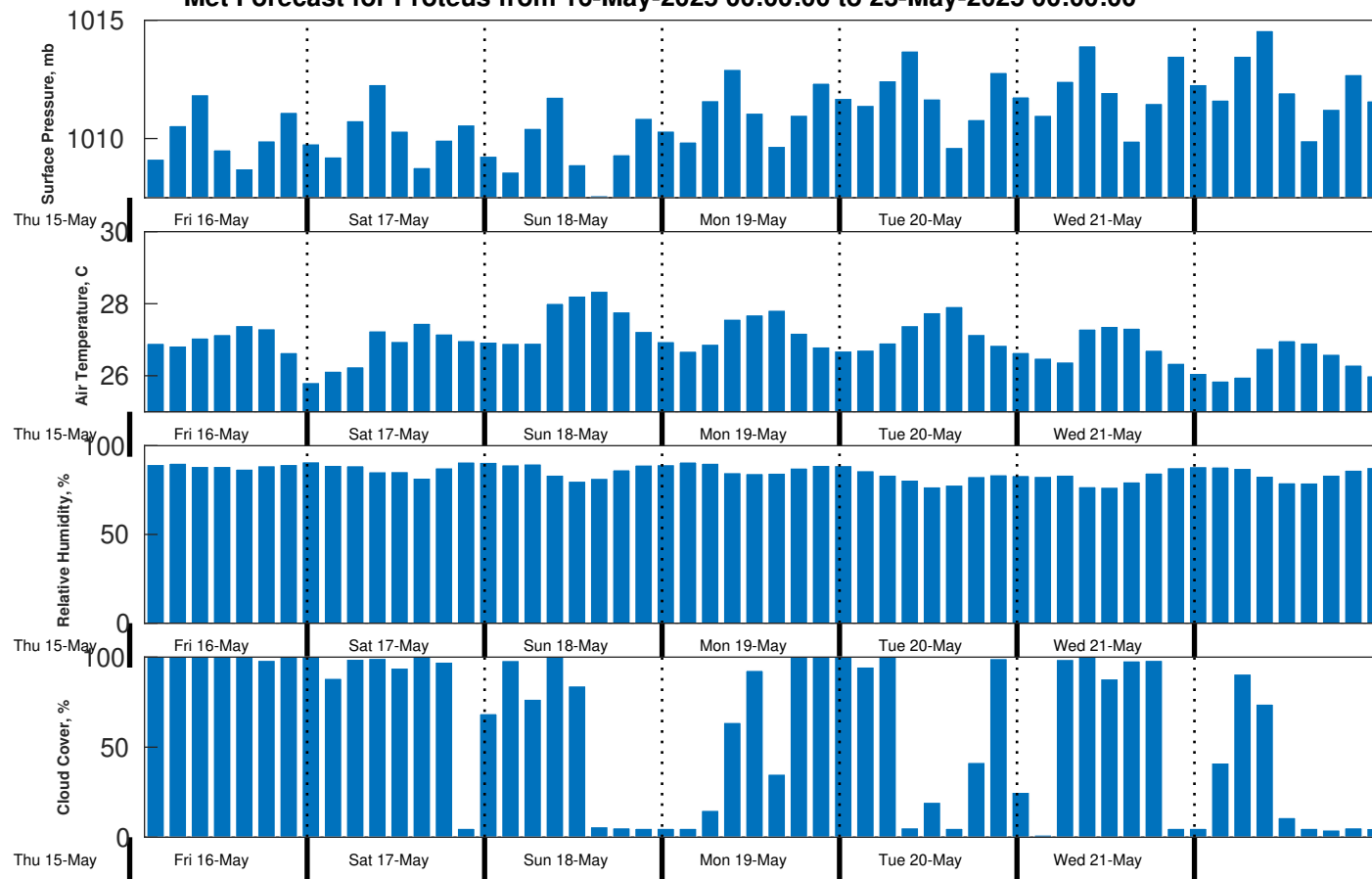
Met Forecast for Proteus from 16-May-2025 00:00:00 to 23-May-2025 00:00:00
