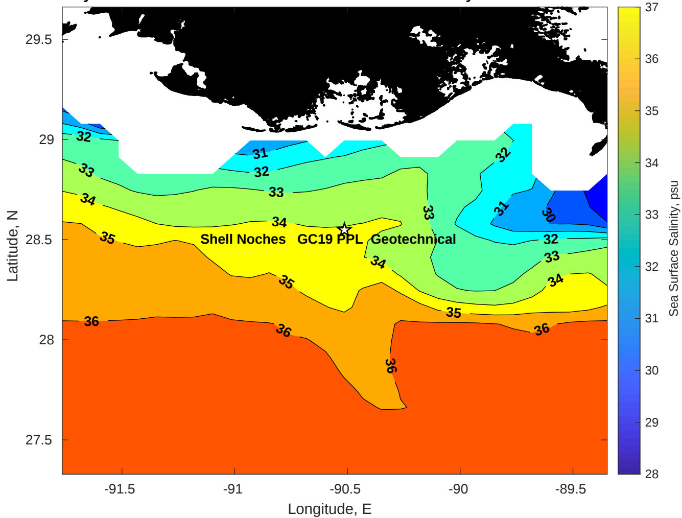
Surface Salinity for Shell Noches GC19 PPL Geotechnical at 15-May-2025 00:00:00
