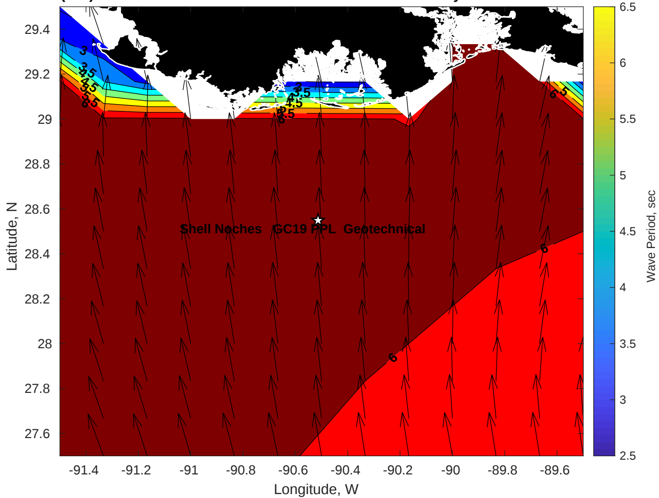
Wave Period (sec) for Shell Noches GC19 PPL Geotechnical at 16-May-2025 09:00:00
