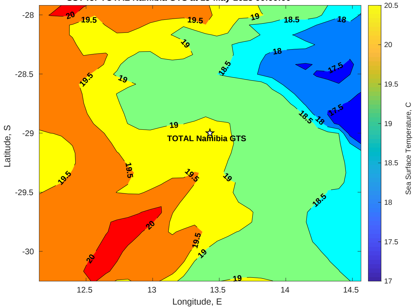
SST for TOTAL Namibia GTS at 15-May-2025 00:00:00
