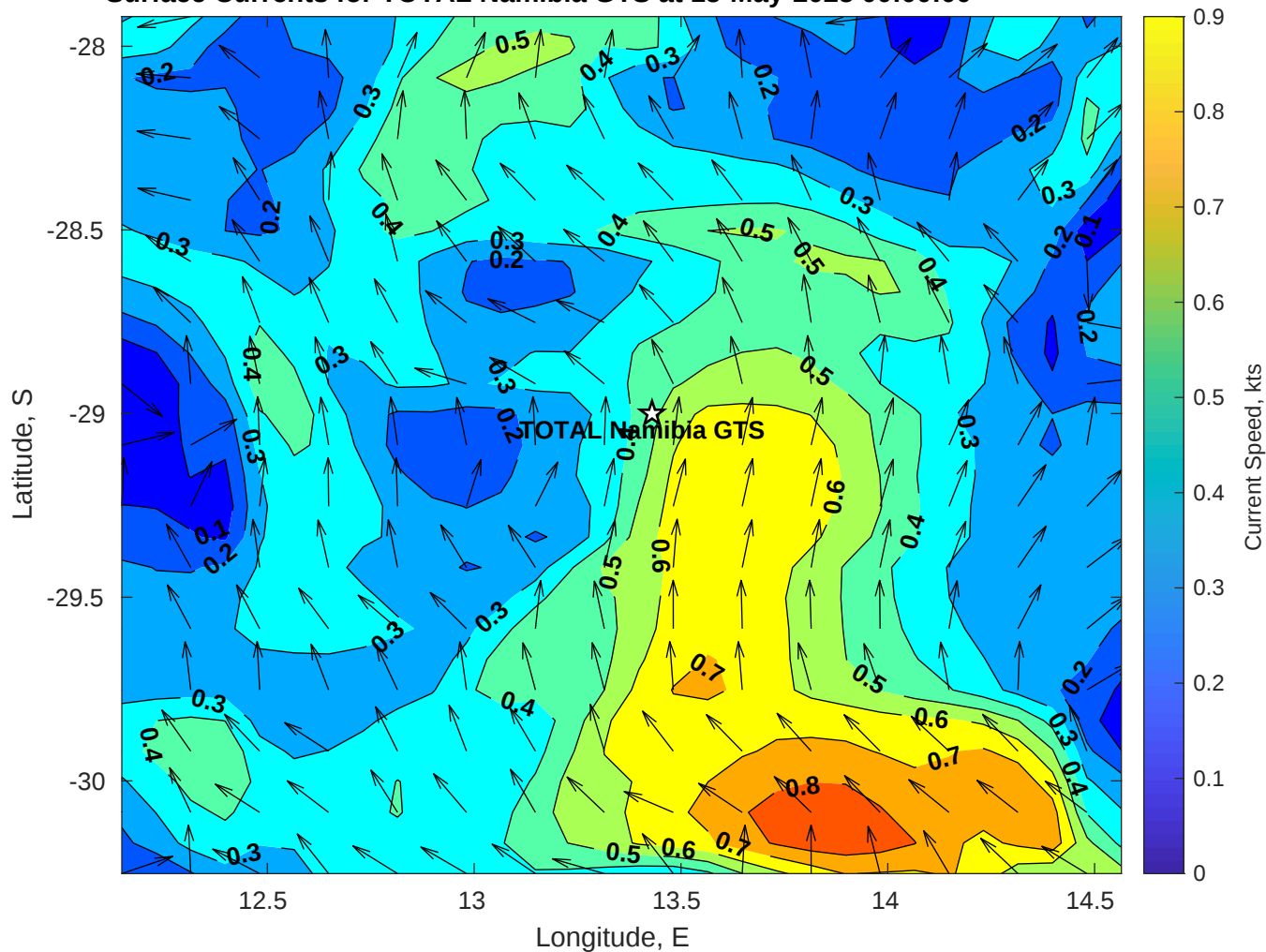
Surface Currents for TOTAL Namibia GTS at 15-May-2025 00:00:00
