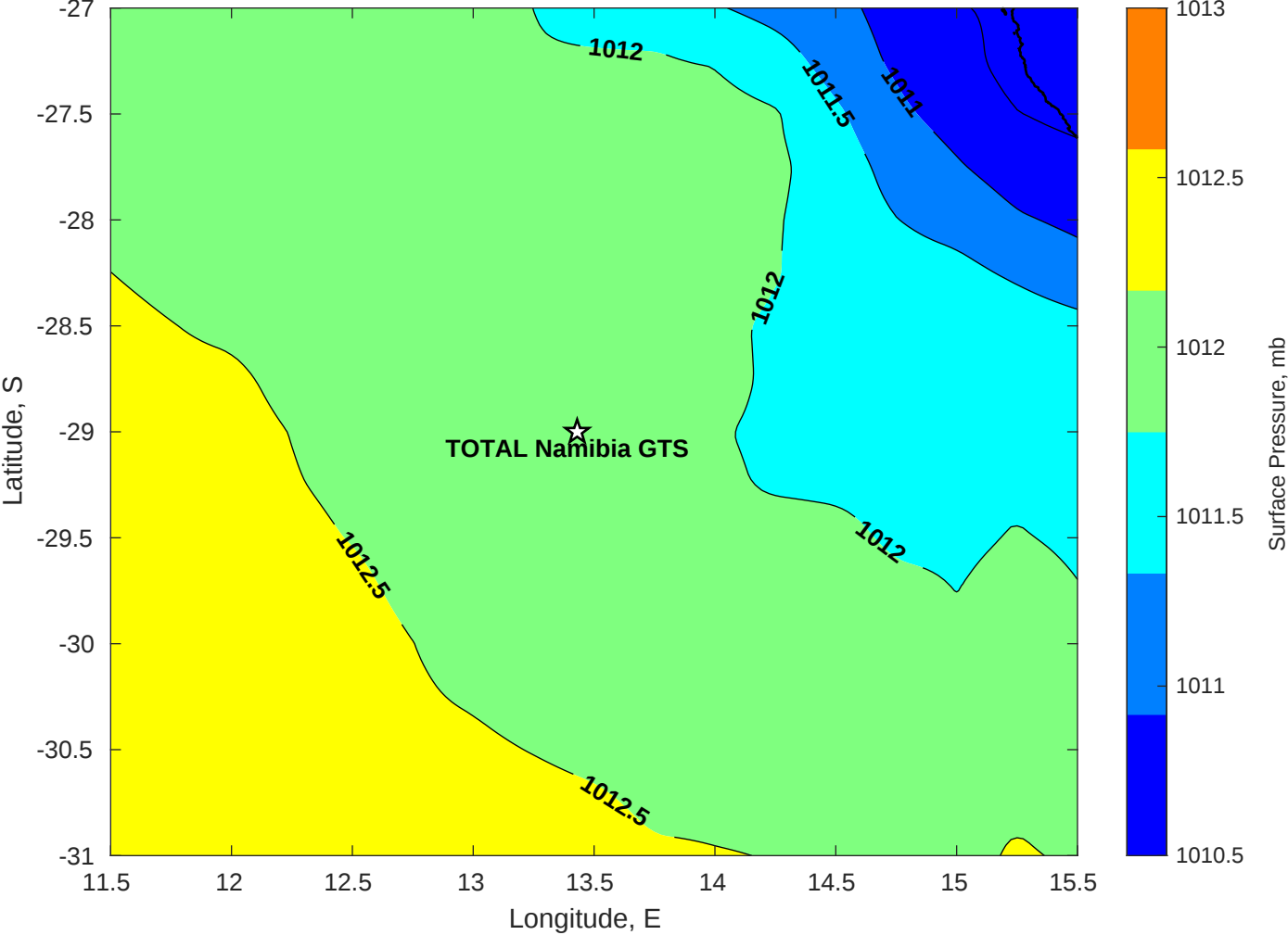
Surface Pressure (mb) for TOTAL Namibia GTS at 17-May-2025 12:00:00
