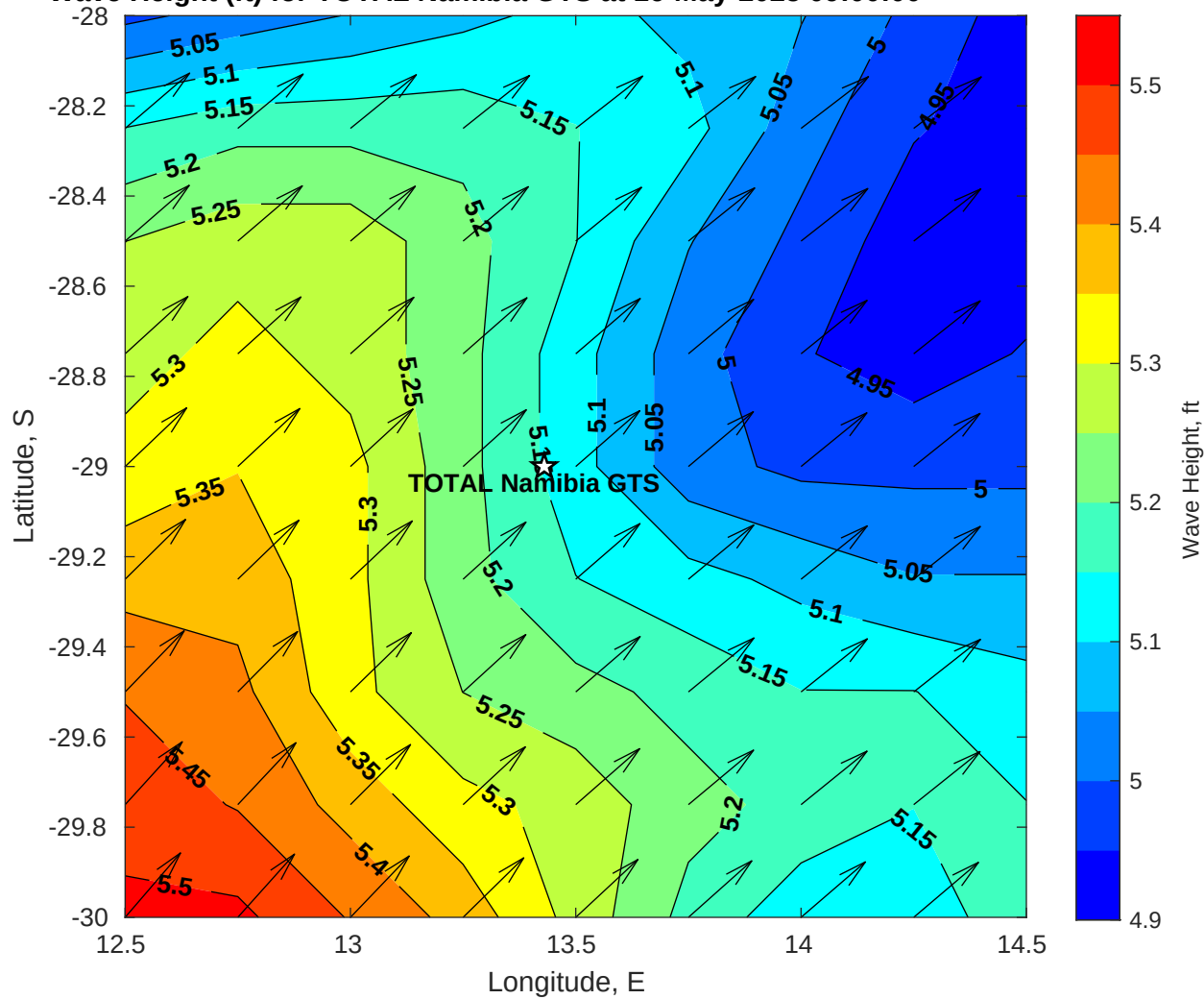
Wave Height (ft) for TOTAL Namibia GTS at 16-May-2025 09:00:00
