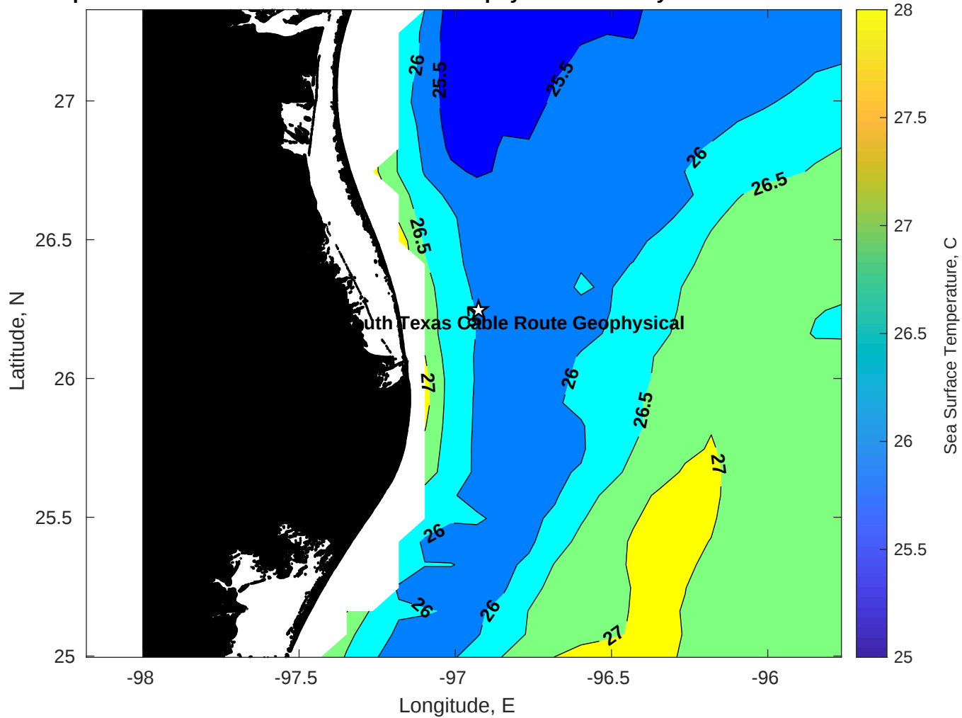
SST for Tampnet P2378 South Texas Cable Route Geophysical at 15-May-2025 00:00:00
