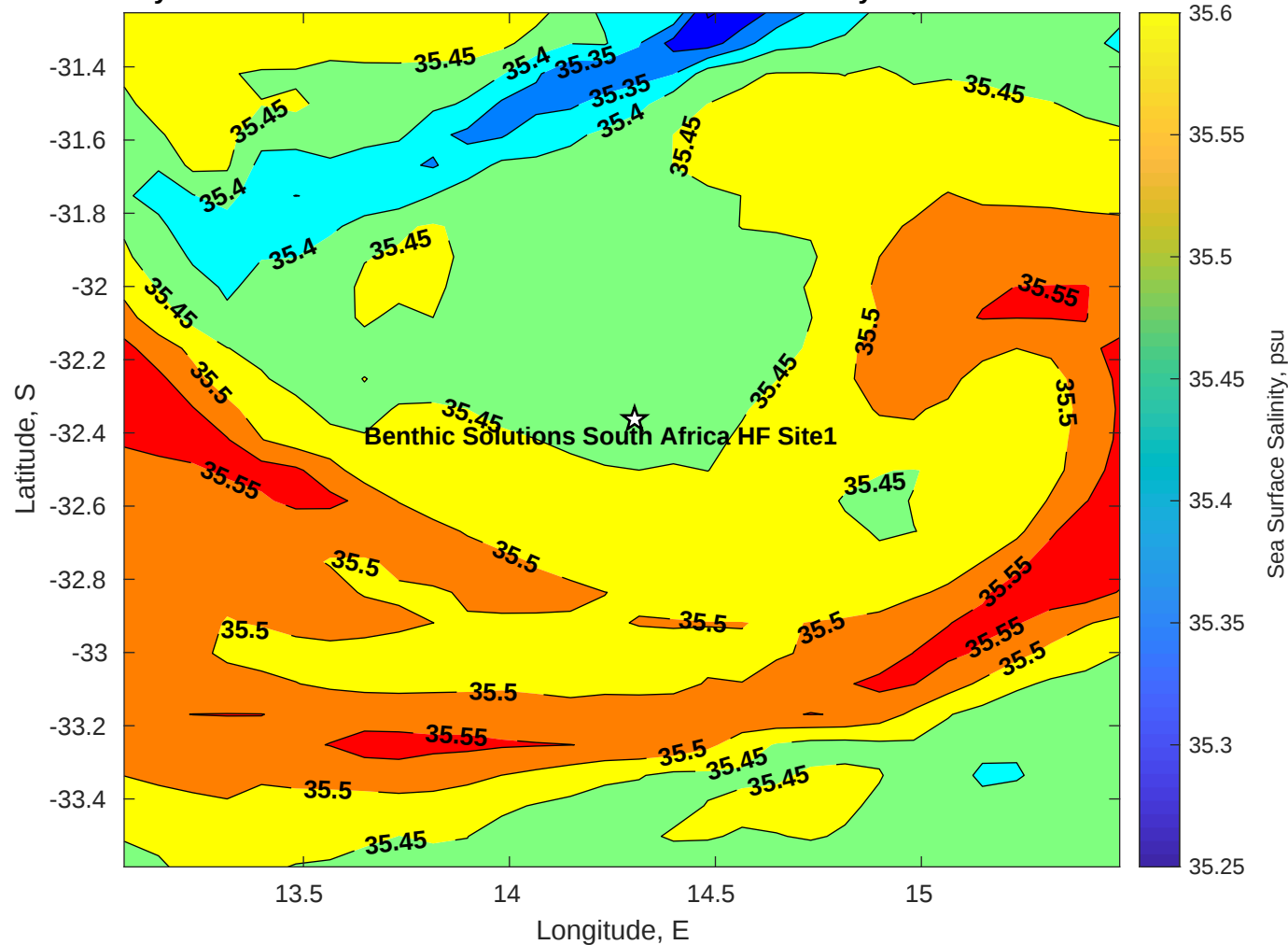
Surface Salinity for Benthic Solutions South Africa HF Site1 at 16-May-2025 00:00:00
