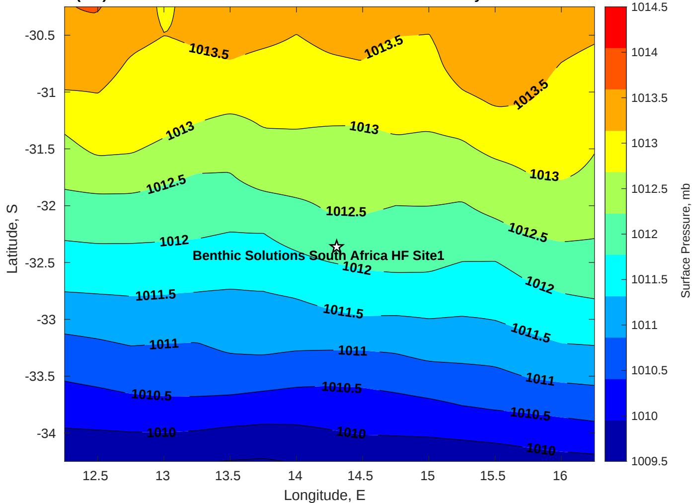
Surface Pressure (mb) for Benthic Solutions South Africa HF Site1 at 19-May-2025 00:00:00
