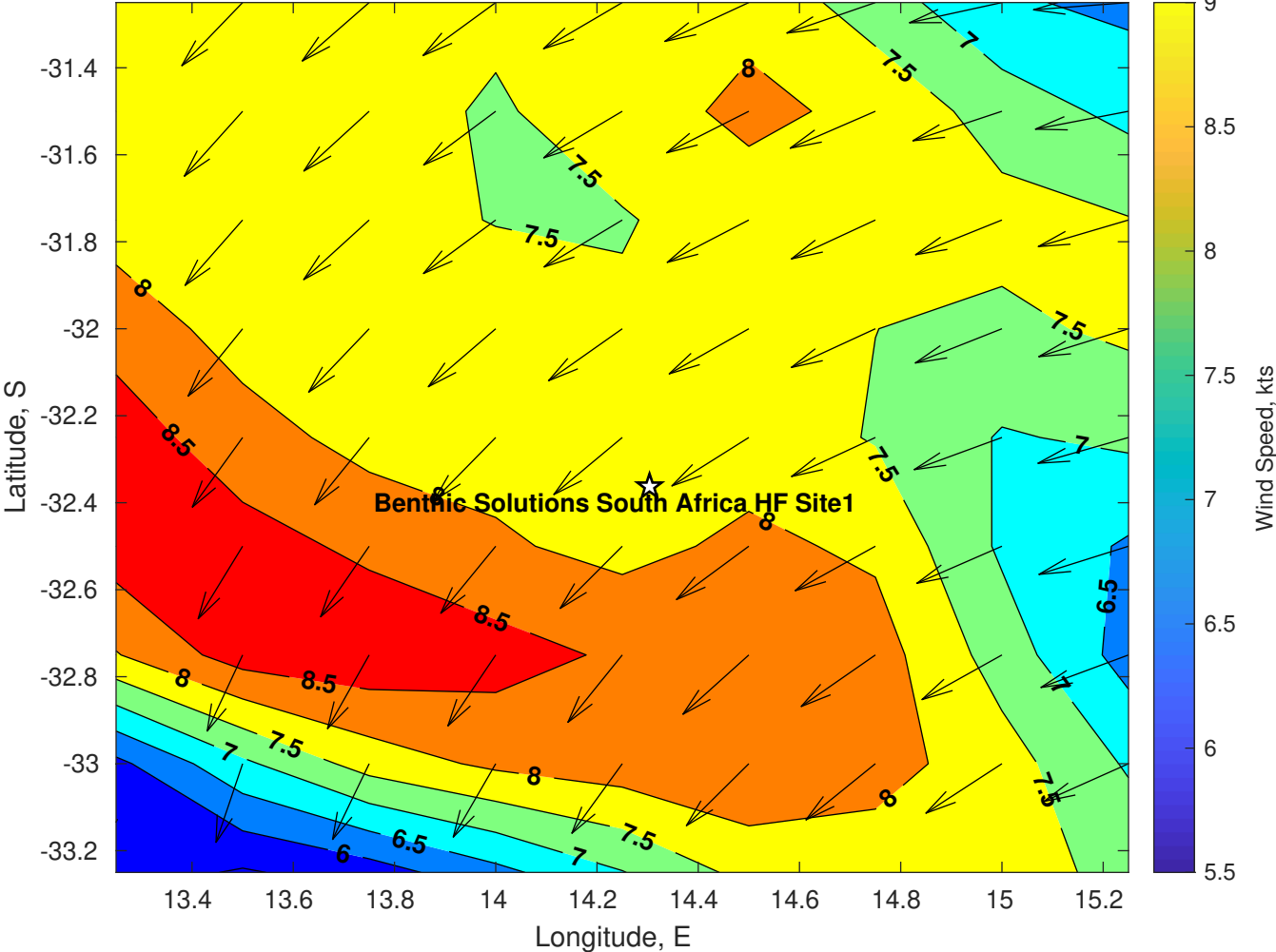
Winds (kts) for Benthic Solutions South Africa HF Site1 at 17-May-2025 09:00:00
